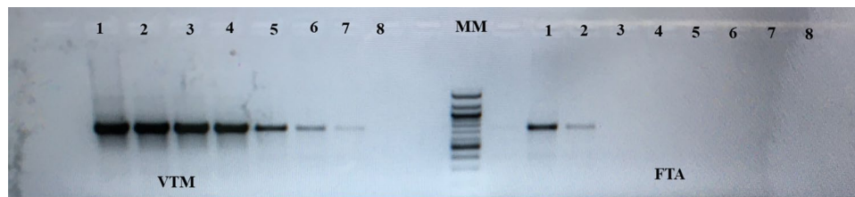
Fig. 3 SARS-CoV-2 RNA recovery from FTA and VTM sample dilutions after ten-fold serial dilution of known positive sample (3.7 × 10 4 copies/μl). Lanes 1–8: dilution corresponding to neat, 10 -1 , 10 -2 , 10 -3 ,
