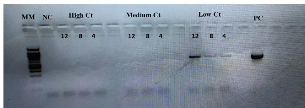
Fig. 2 Detection of SARS-CoV-2 RNA (ORF-8 gene; 777bp) on FTA cards in three categories of samples (High Ct, Medium Ct and Low Ct values) done by punching 4, 8 and 12 disks. MM-Molecular Marker (100 bp); NC-Negative Control; PC-Positive Control
