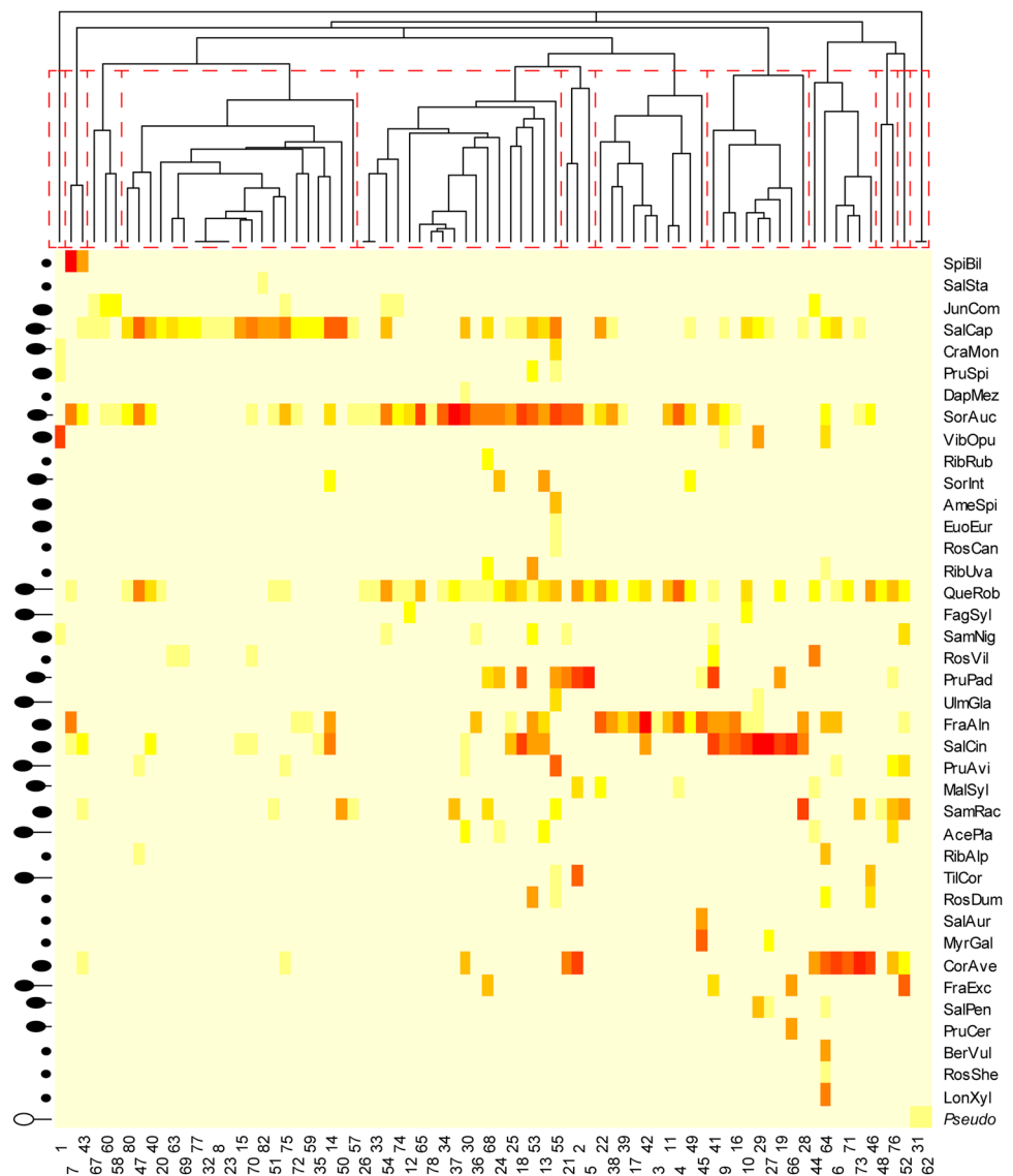
Fig. 5 Heatmap of the UPGMA clustering for the idealized management set. Grouping and dendrogram at the top, abbreviated species to the right (see Table 2), and site numbers at the bottom. The darkest color (red) indicates the highest abundance and the brightest (yellow) the lowest abundance. General growth form of species as small shrub, large shrub, shrub tree/small tree, and tree is graphically illustrated to the left
