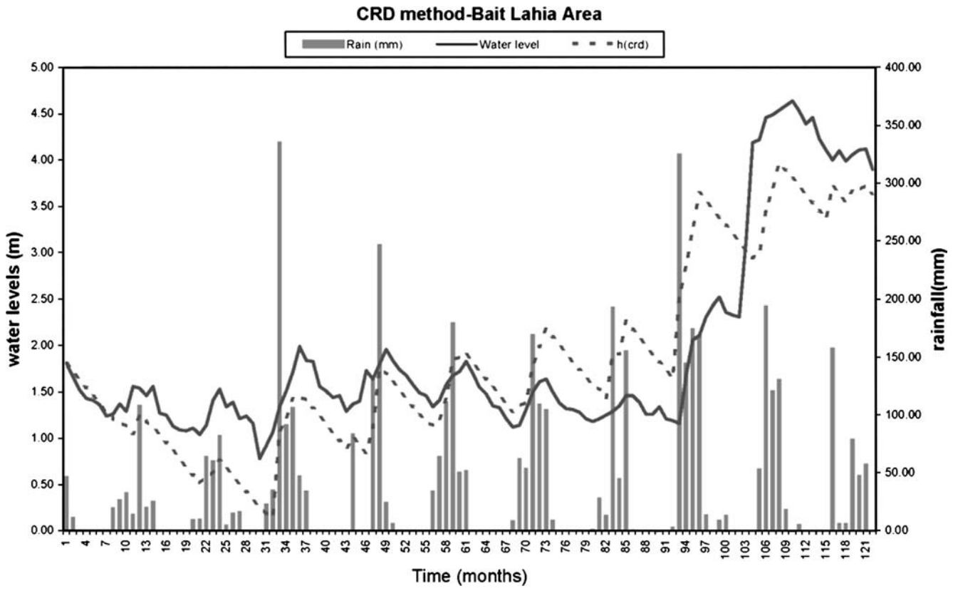
Fig. 5 CRD fitting diagram for Bait Lahia area
