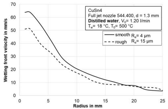
Fig. 16 Effect of roughness on wetting front propagation with full jet nozzle
