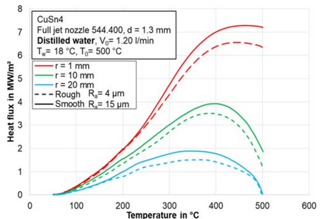
Fig. 17 Boiling curves for distilled water with full jet nozzle
