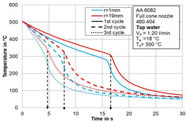
Fig. 8 Temperature curves for repeated cooling cycles with local tap water
