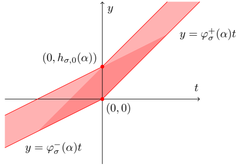
Fig. 2. The mass-growth y = h_{\sigma,t}(\alpha) lies in the red shaded region, and in the pale red shaded region when there is an algebraic stability condition in the component of \sigma —see Proposition 3.2 (colour figure online)
