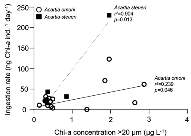
Fig. 9 Correlation between ingestion rate and micro-phytoplankton (> 20 \mu\text{m} ) biomass (Chl- a concentration) for adults of Acartia species ( Acartia omorii and A. steuerei )
