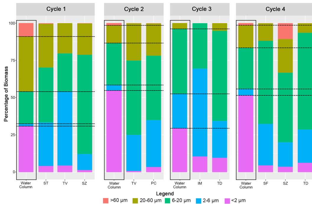
Fig. 3 Contribution of particles of various size classes to the total biomass present in the water column (outlined by black boxes) compared to that of the guts of each of the 58 salps sampled averaged by species (as indicated on the x-axis) per cycle. WC water column, SF
