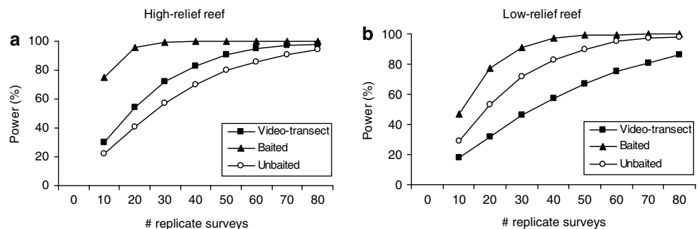
Fig. 2 The power of stereo-video transects, baited and unbaited remote stereo-video techniques to detect a 25% change in the mean total number of individuals ( \alpha=0.05 ) at a high-relief reef and b low-relief reef sites
