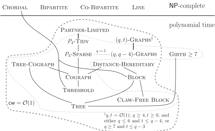
Fig. 1 Some graph classes on which the complexities of b -COLORING and b -CHROMATIC NUMBER problem were studied. Whenever two classes are connected by a line, the upper one contains the lower one. All NP-hardness results hold for b -CHROMATIC NUMBER and all polynomial time results, except the one for graphs of girth at least seven, hold for b -COLORING. The inner bottom area (dotted line) shows classes for which polynomial time algorithms were previously known and the outer area (dashed line, labeled cw = \mathcal{O}(1) ) shows on which classes our algorithm can be applied
