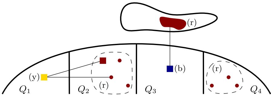
Fig. 3 Illustration of the definition of a color class being of a certain t -type inside a partial b -coloring of G_t . The large square vertices are partial b -vertices for their color. The type of the red (r) color in the coloring is as follows. Since it has a b -vertex (the one in Q_2 ), we have that \xi = 1 . Since Q_2 and Q_4 have red vertices, \phi(Q_2) = \phi(Q_4) = \text{cont} . Q_1 and Q_3 do not have red vertices. Q_1 contains the b -vertex of color yellow (y), but this vertex already has a red neighbor. Therefore, \phi(Q_1) = \text{none} . Finally, Q_3 has the b -vertex of color blue (b), and this vertex does not have a red neighbor yet. Therefore, there has to be a red vertex among the future neighbors of Q_3 . Hence, \phi(Q_3) = \text{dem}
