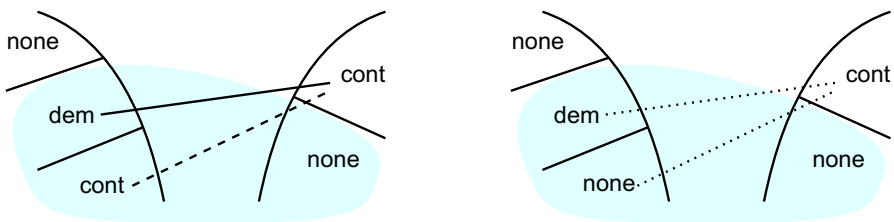
Fig. 4 Illustration of Definition 3.5. The shaded area shows a bubble and the labels on the equivalence classes correspond to type labelings. For the left hand side, note that between a pair of classes that are both labeled ‘cont’, there can be no edge in the operator. Moreover, since the bubble contains a class labeled cont and one labeled dem, the demand of the latter has to be fulfilled at this node, i.e. there has to be an edge from this class to a ‘cont’-class. The right side shows the situation when the ‘cont’-class in the bubble is changed to ‘none’, in which case the dotted edges may or may not be present in the operator.
