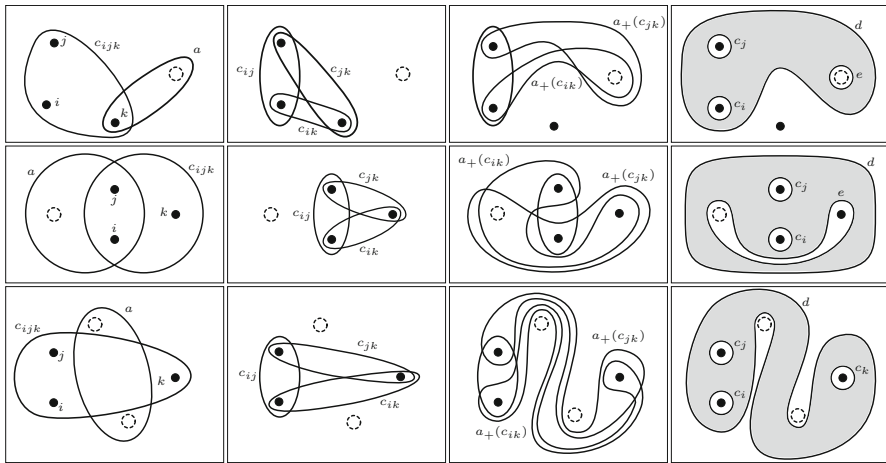
Fig. 8 The curves and four-holed spheres used in the proof of Lemma 4.12. From top to bottom, the rows correspond to the cases where A \cap \{i, j, k\} is \{k\} , \{i, j\} , and \emptyset , respectively. The dotted circles contain unspecified numbers of marked points
