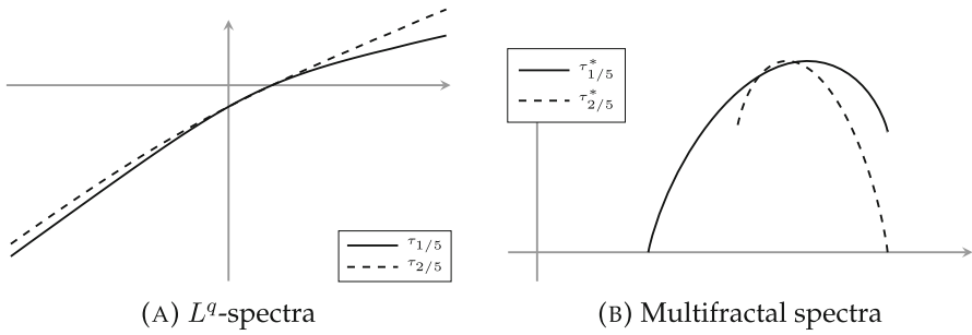
Fig. 2. L^q -spectra and multifractal spectra corresponding to a recognisable substitution for p \in \{1/5, 2/5\}
