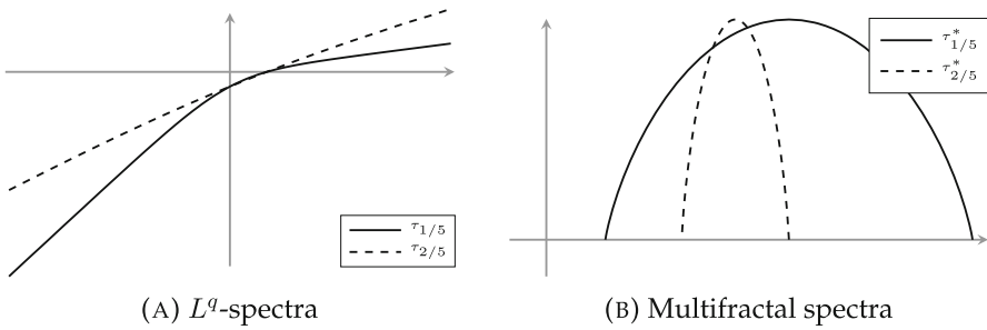
Fig. 1. L^q -spectra and multifractal spectra corresponding to a recognisable substitution for p \in \{1/5, 2/5\}
