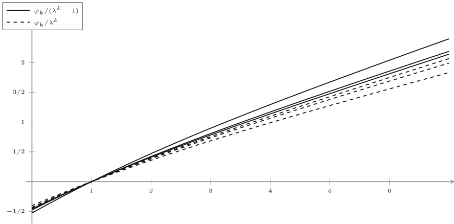
Fig. 3. Upper and lower bounds on the L^q -spectrum of the frequency measure corresponding to the random Fibonacci substitution with p = 1/2 , for k = 3, 5, 7 . The darker shades correspond to higher values of k
