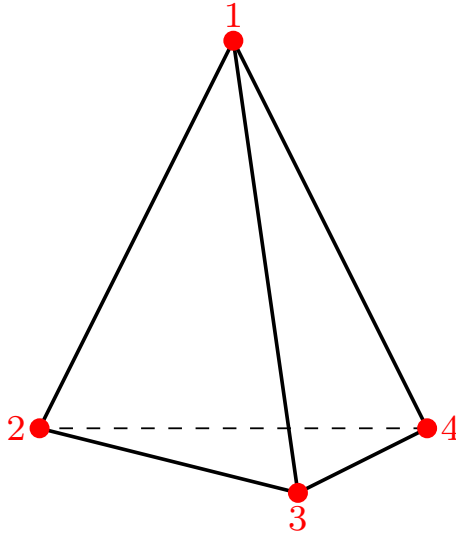
Fig. 1. A tetrahedron with the sets \underline{4} and \underline{4}^\vee associated with vertices and faces, respectively. Each vertex is labeled by a \in \underline{4} and represents a complex plane \mathbb{C}_a . The edge connecting two vertices labeled by a and b represents a complex two-plane \mathbb{C}_{ab}^2 = \mathbb{C}_a \times \mathbb{C}_b . The face A = (abc) \in \underline{4}^\vee has three vertices a, b, and c, and represents a complex three-plane \mathbb{C}_A^3 = \prod_{a \in A} \mathbb{C}_a . The remaining vertex that is not in the face A \in \underline{4}^\vee is denoted by \check{A} \in \underline{4}
