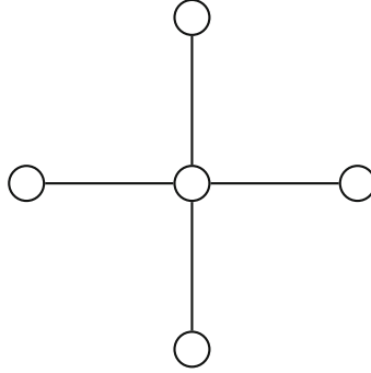
Fig. 10. A star-shaped graph (here with m = 4 peripheral nodes)
