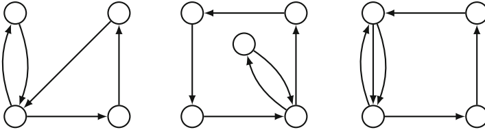
Fig. 8. Cycles with opposite arrows which arise as necklace Lie brackets of isomonodromy cycles: first list
