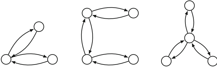
Fig. 9. Cycles with opposite arrows which arise as necklace Lie brackets of isomonodromy cycles: second list
