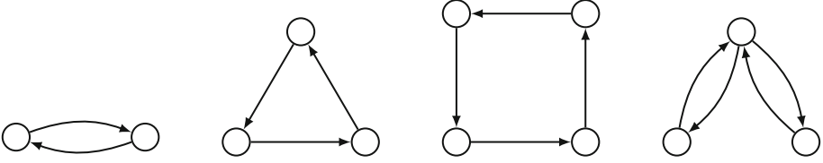
Fig. 1. Isomonodromy cycles
