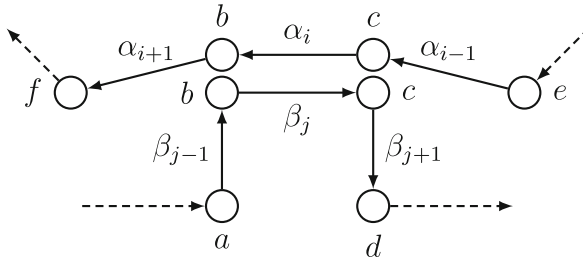
Fig. 2. Cut-and-glue rule for the necklace Lie bracket: before cutting a pair of opposite arrows
