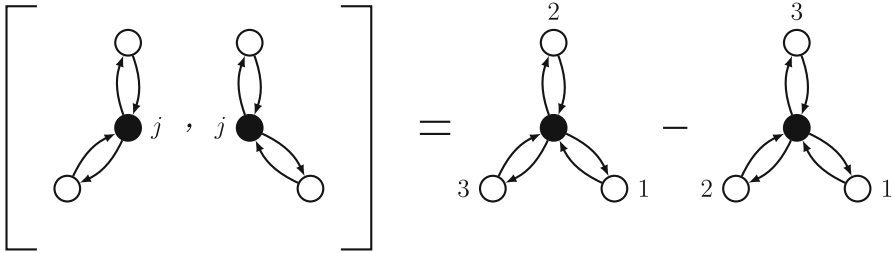
Fig. 7. Commutator of two degenerate quantum 4-cycles with centres in common (the numbers at the peripheral nodes indicate the order in which they are touched)
