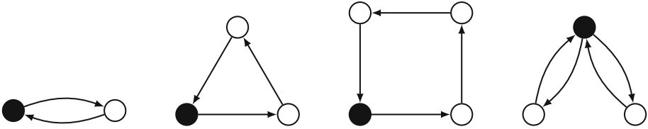
Fig. 5. Quantum isomonodromy cycles
