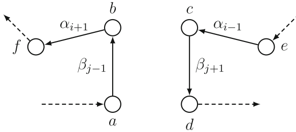
Fig. 3. Cut-and-glue rule for the necklace Lie bracket: after cutting a pair of opposite arrows
