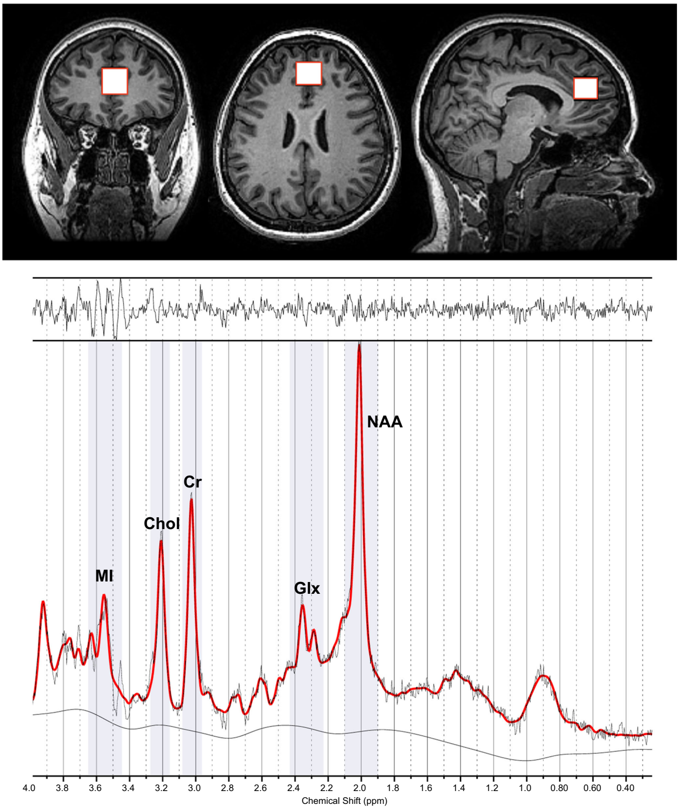
Fig. 1 ^1\text{H} -MRS voxel position and example spectra in the anterior cingulate cortex. NAA, N -acetylaspartate; Glx, glutamate + glutamine; Cr, creatine; Chol, choline; MI, myo-inositol
