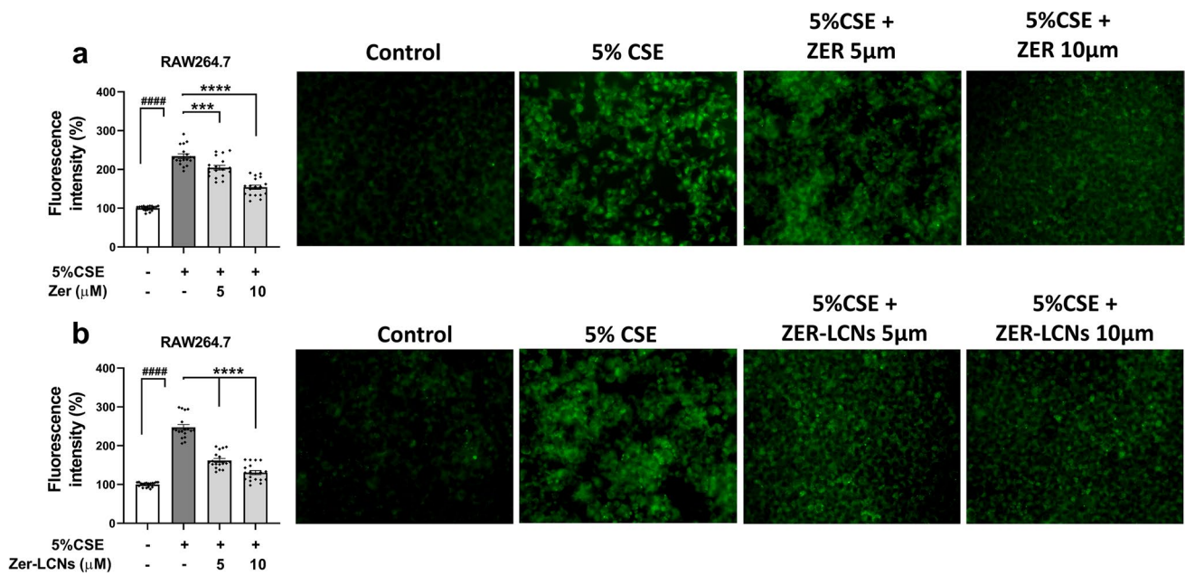
Fig. 3 Effect of free ZER and ZER-LCNs on ROS production in RAW264.7 cells. RAW264.7 cells were pre-treated for 1 h with or without ZER (a) or ZER-LCNs (b) at final concentration of 5 and 10 \mu\text{M} , followed by 24 h incubation in the absence or presence of 5% CSE. The fluorescence intensity of DCF-DA was measured using fluorescence plate reader and the fluorescence images were acquired using fluorescence microscopy at \times 20 magnification. Values are
