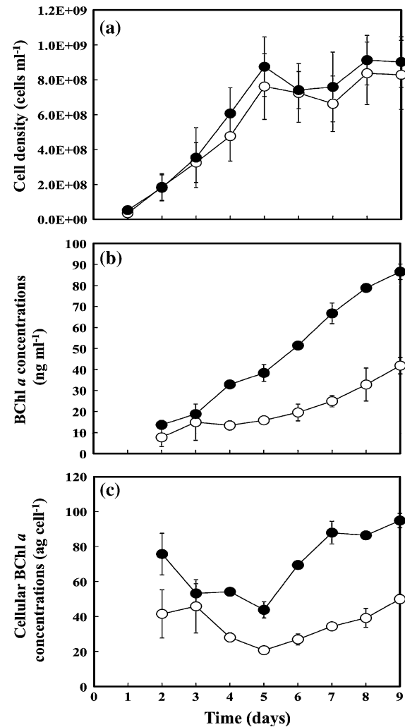
Fig. 2 Changes over time in the a cell densities, b BChl a concentration, and c cellular BChl a levels of OBYS 0001 (filled circle) and NBRC 14126 (open circle)
