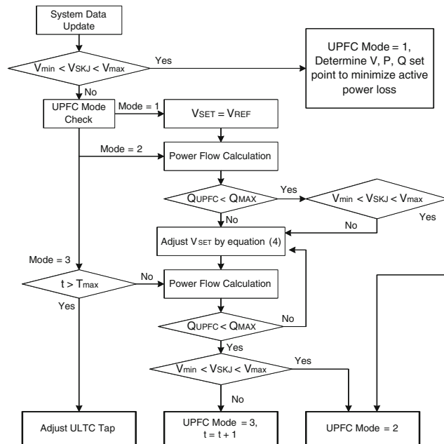
Fig. 5 Flowchart of the operation algorithm in the normal state
