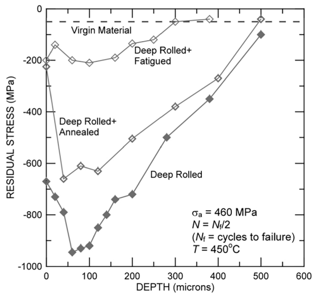
b Surface residual stress affected by fatigue cycling
