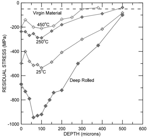
a Surface residual stress affected by temperature
