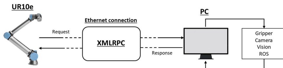
Fig. 6 Communication system between the UR robot and the PC
