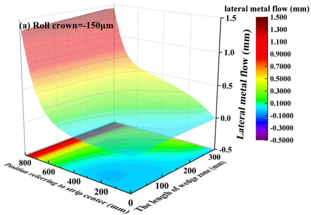
◀ Fig. 15 Lateral spread curves for different roll crowns: a roll crown = -150\mu\text{m} ; b roll crown = -100\mu\text{m} ; c roll crown = -50\mu\text{m} ; d roll crown = 0\mu\text{m}
