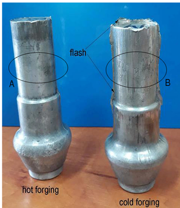
Fig. 11 Shaft forgings obtained in the experimental tests
