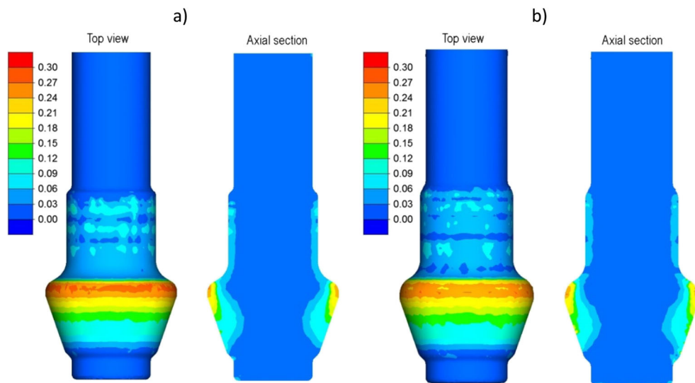
Fig. 9 Distribution of the Cockcroft–Latham ductile fracture criterion: (a) cold forging and (b) hot forging
