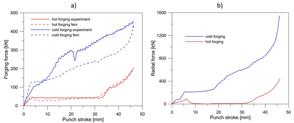
Fig. 10 Force curves of the forging process: (a) forging force and (b) radial force
