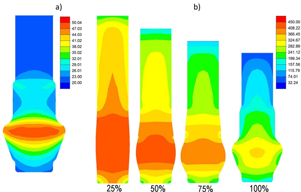
Fig. 7 Temperature distribution (°C) in shaft: (a) cold forging and (b) hot forging
