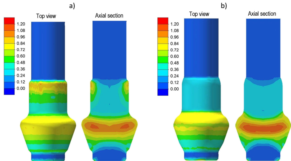
Fig. 4 Distribution of effective strain in shaft after: (a) cold forging and (b) hot forging
