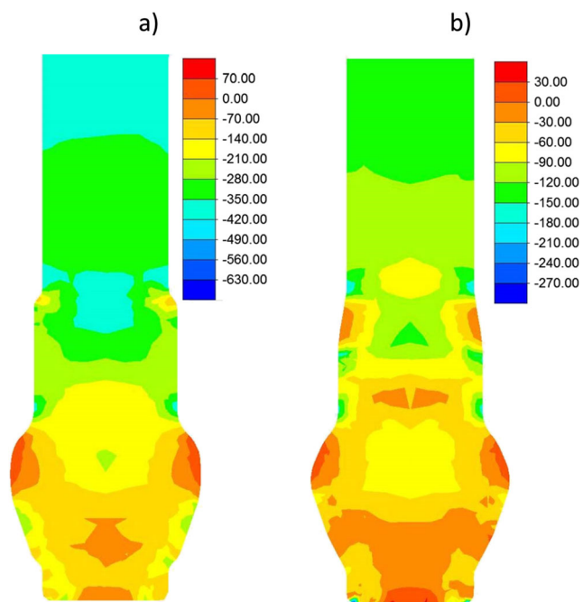
Fig. 8 Distribution of mean stress (MPa): (a) cold forging and (b) hot forging
