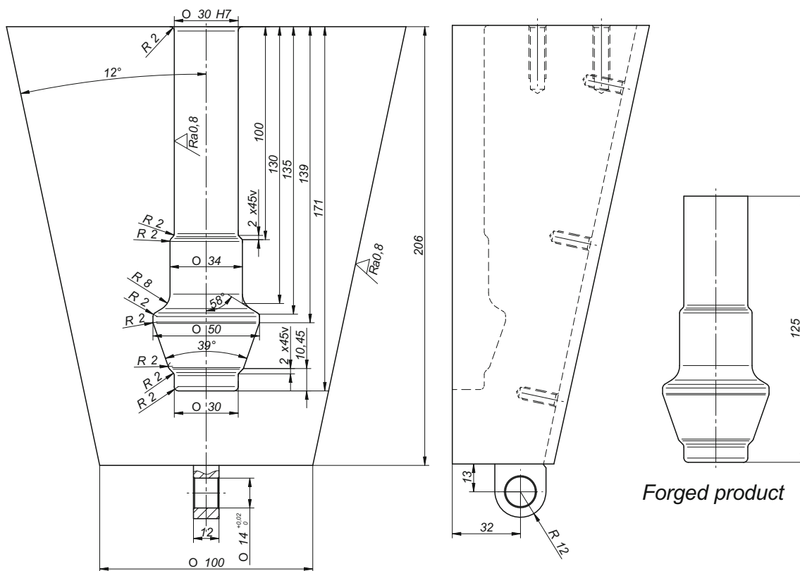
Fig. 1 Vertical split die for forging a stepped shaft
