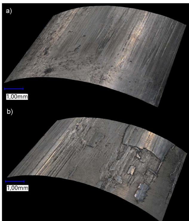
Fig. 12 Shaft surfaces magnified 20x: (a) the A area of the hot-forged shaft and (b) the B area of the cold-forged shaft
