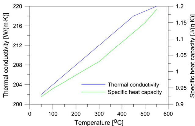
Fig. 3 Thermal parameters of AW-6060 aluminum used in FEM modeling
