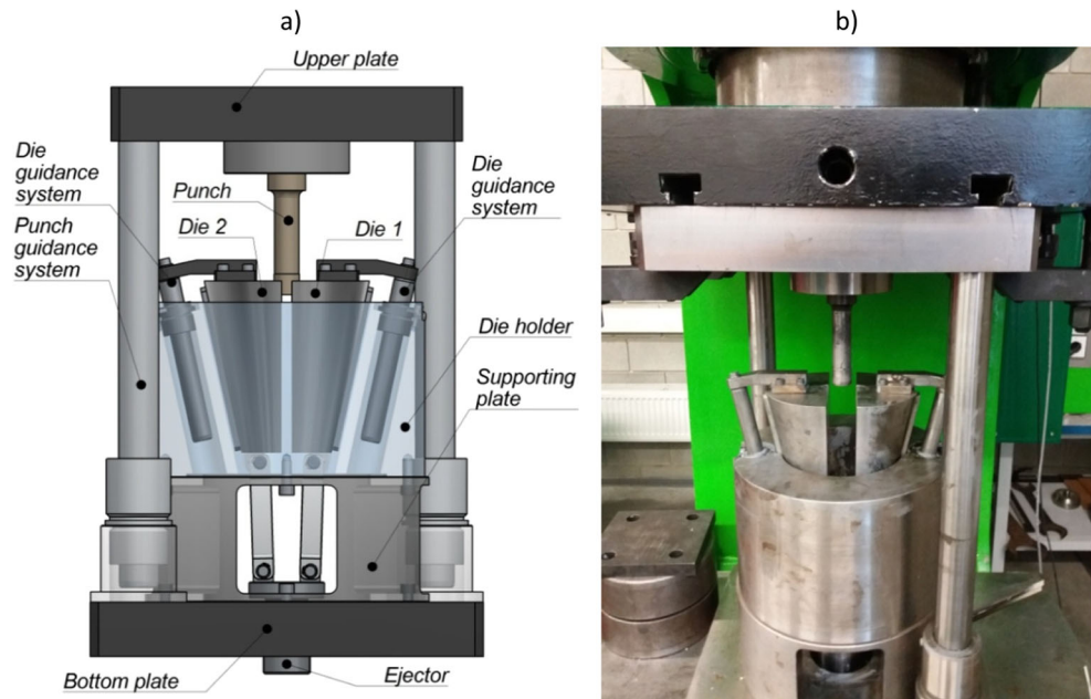
Fig. 2 A forging device with a vertical split die: (a) CAD model and (b) real view
