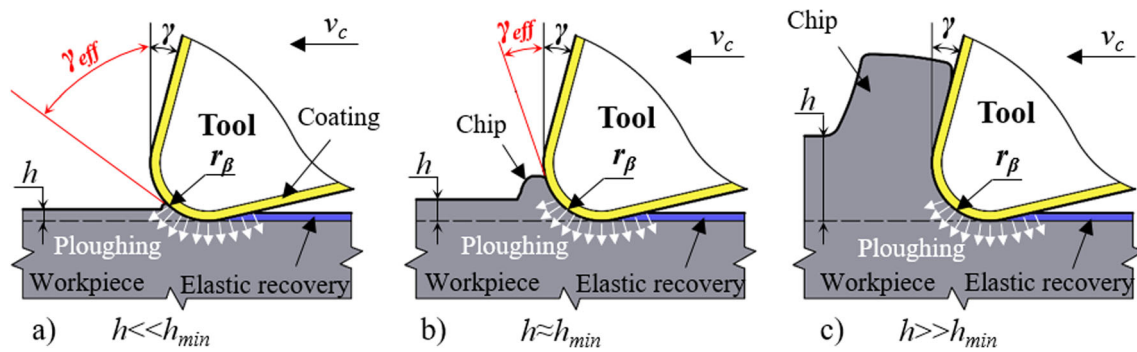
Fig. 1 Schematic of micro-chip removal mechanisms: (a) the undeformed chip thickness ( h ) is smaller than the minimum chip thickness ( h_{min} ), (b) the value of h is comparable to the value of h_{min} , (c) the value of h is higher than the value of h_{min} (adapted from [42, 72])
