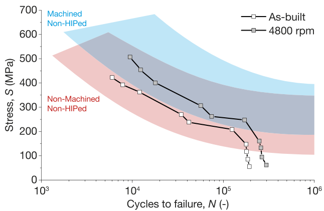
Fig. 13 S-N curve for as-built samples and treated samples (4800 rpm for 10 h) and in the background typical fatigue ranges of non-HIPed machined and non-machined samples according to Chern et al. [31]
