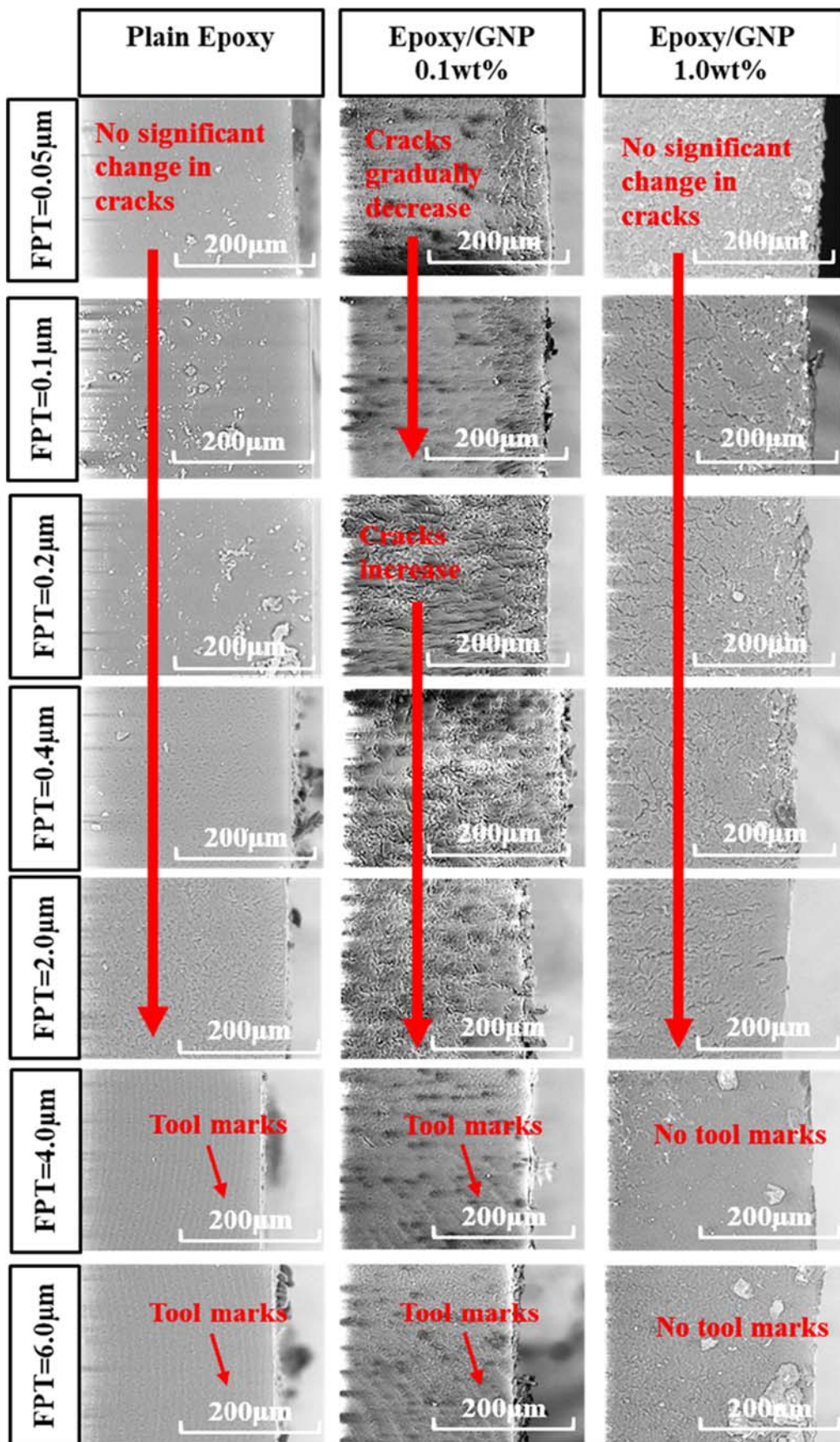
Fig. 8 SEM images of slot bottom surfaces for FPT values between 0.05 and 6.0 \mu m
