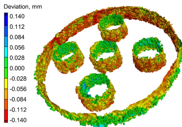
Fig. 9 Distribution of the deviations of sample C (measured by \mu CT) with respect to the CAD model shown as color-coded map of deviations
