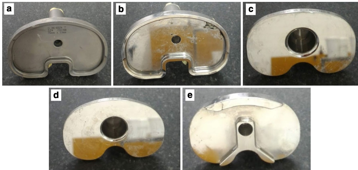
Fig. 1 Examples of two designs and relative iterations involved in the study: a Ti PFC fixed bearing, b CoCr PFC fixed bearing, c CoCr PFC RP, d Attune rotating bearing, e Attune fixed bearing
