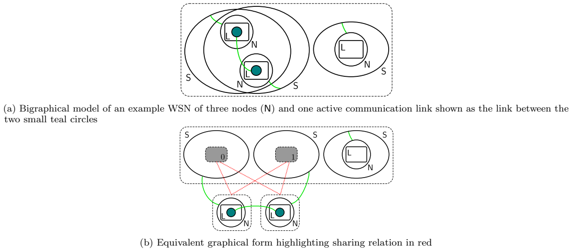
Fig. 8. Example Bigraph representing a WSN
