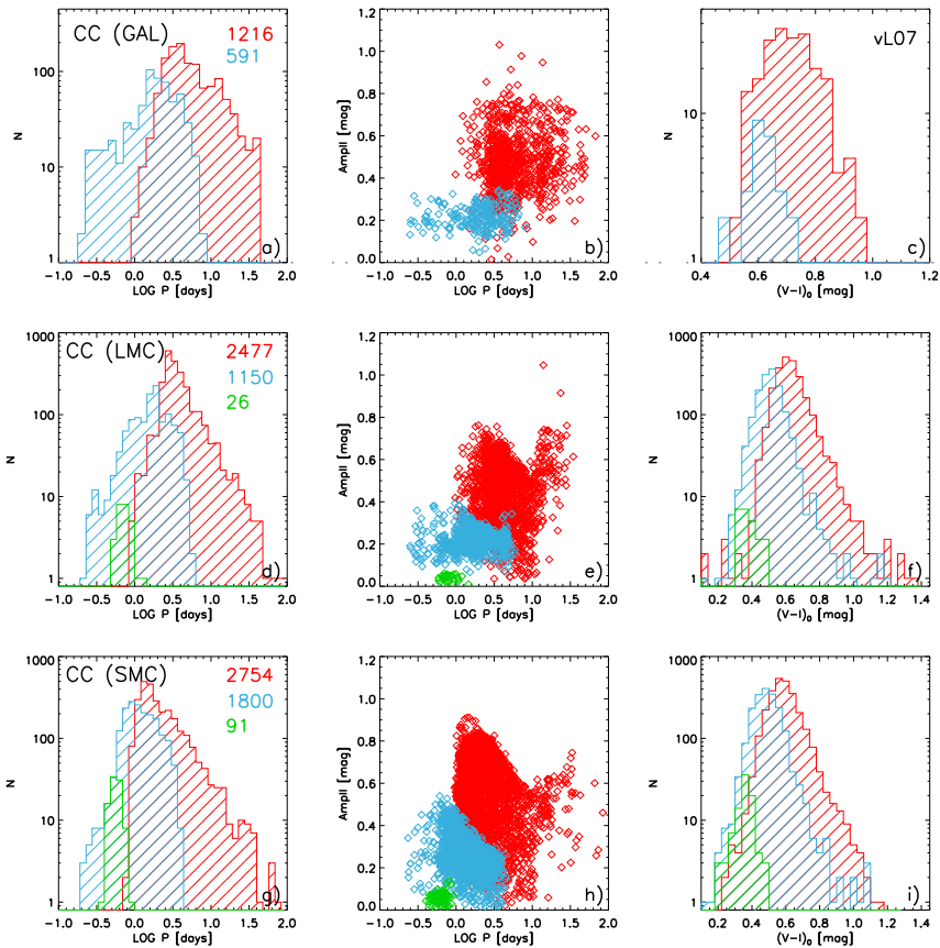
Fig. 3 Top: a Period distribution for fundamental (red hatched area), and first overtone (light blue hatched area) Galactic CCs. Note that the Y-axis is logarithmic. b I -band luminosity amplitude versus logarithmic period (Bailey diagram) for FU (red), and FO (light blue) Galactic CCs. c Dereddened (V - I)_0 color distribution for CCs. The sample adopted for the color distribution is based on multi-band optical photometry provided by van Leeuwen et al. (2007, vL07) and on individual reddenings provided by Tammann et al. (2003). Middle: Same as the top, but for LMC CCs ( d–f ). The green hatched area shows the period distribution of second overtone CCs. Bottom: Same as the middle, but for SMC CCs ( g–i )
