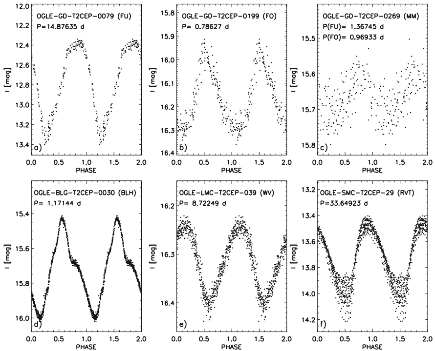
Fig. 8 a Light curve for a Galactic TIIC pulsating in the fundamental mode from the OGLE IV data set. The ID and the period are labelled. b Same as a , but for a Galactic first overtone TIIC. c Same as a , but for a Galactic mixed-mode TIIC. Primary and secondary periods are labelled. d Same as a , but for a Galactic Bulge BL Herculis. e Same as a , but for a LMC W Virginis. f Same as a , but for a SMC RV Tauri
