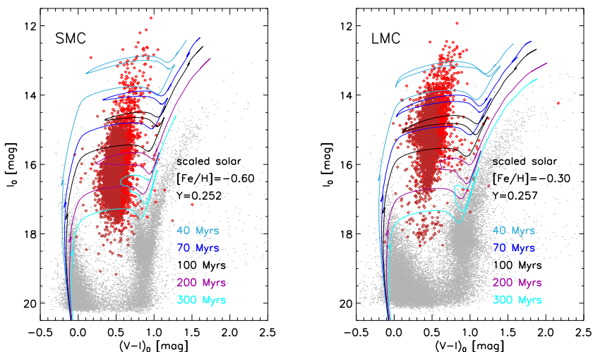
Fig. 13 Left: Comparison between theory and observations in the dereddened I_0 , (V - I)_0 CMD for SMC CCs. CCs are marked with light (fundamental) and dark (first overtone) red symbols, while static stars with grey dots. Variable stars were dereddened using the reddening map provided by Skowron et al. (2021), while static stars were dereddened through a mean reddening of E(V - I) = 0.047 mag (Skowron et al. 2021). Solid lines display selected scaled-solar stellar isochrones from the BASTI-IAC database at a fixed chemical composition ( [Fe/H] = -0.60 , Y = 0.252 ) and ages ranging from 30 to 300 Myrs (see labelled values). Isochrones were plotted by assuming a true distance modulus of \mu = 18.977 \pm 0.028 mag (Graczyk et al. 2020). Right: Same as the left, but for LMC CCs and more metal-rich scaled-solar stellar isochrones ( [Fe/H] = -0.30 , Y = 0.257 ). Isochrones were plotted by assuming a true distance modulus of \mu = 18.477 \pm 0.023 mag (Pietrzyński et al. 2019). The mean reddening adopted for static stars is E(V - I) = 0.100 mag (Skowron et al. 2021)
