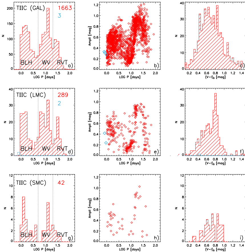
Fig. 9 Top: a Period distribution for fundamental (red hatched area) and first overtone (light blue hatched area) Galactic TIICs. b I-band luminosity amplitude versus period (Bailey diagram) for both FU and FO TIICs. c Dereddened (V - I)_0 color distribution for the same TIICs plotted in the left and in the middle panel. Middle: Same as the top, but for LMC TIICs. Bottom: Same as the top, but for SMC TIICs
