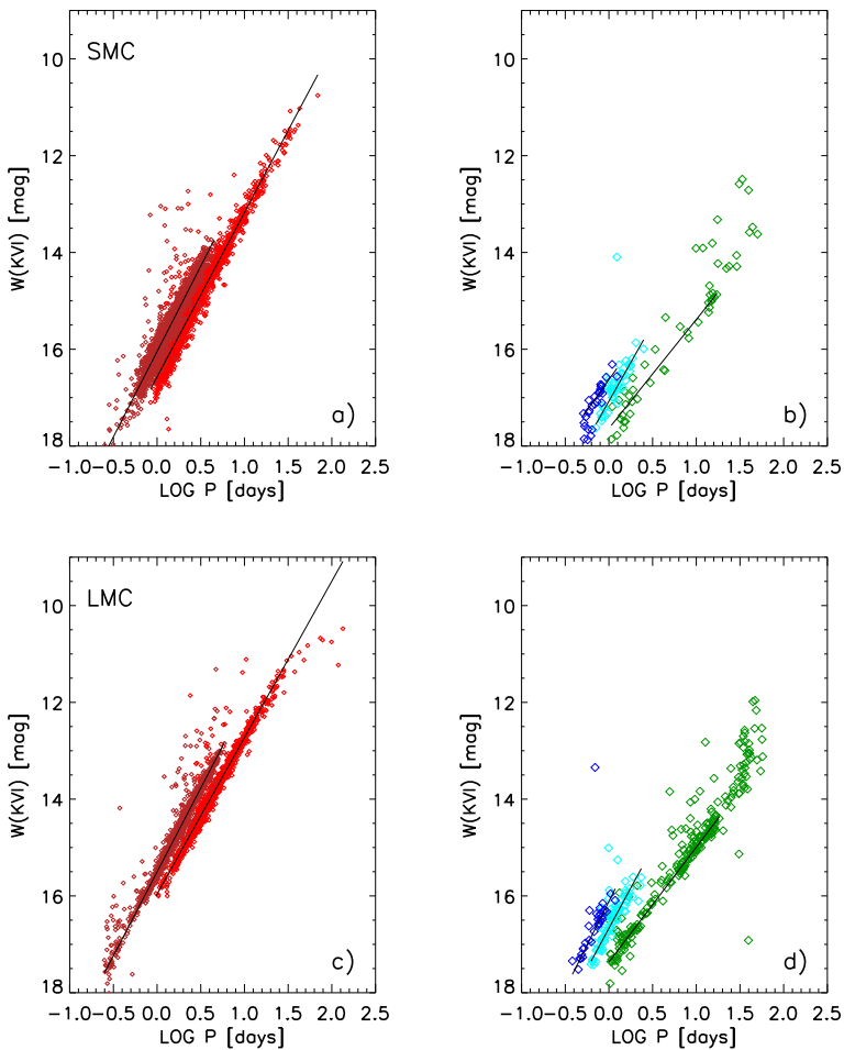
Fig. 19 Top: Optical–NIR, triple-band K , V - I PW relations (see Table S2 of the Supplementary Information) for SMC CCs (a) and for ACs plus TIICs (b). Symbols and color coding are the same as in Fig. 16. Bottom: Same as the top, but for LMC Cepheids (CCs) (c); ACs plus TIICs (d)
