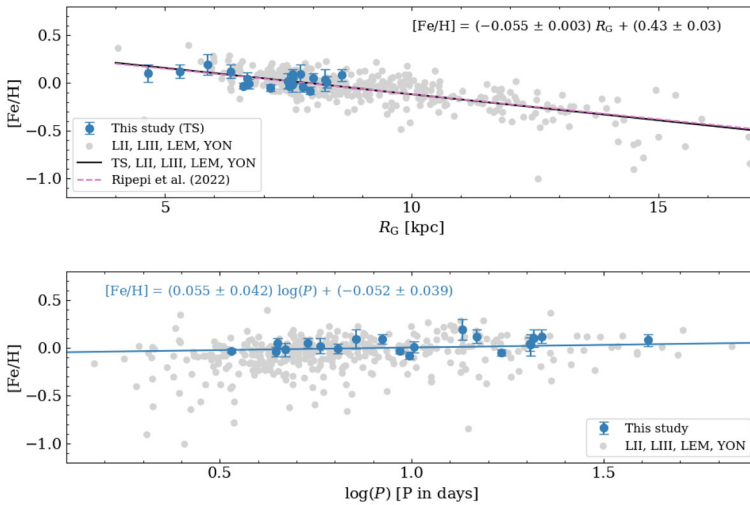
Fig. 25 Top: Iron abundances as a function of the Galactocentric distance for a sample of 20 calibrating Cepheids (blue circles) compared with results from the literature (gray circles): Luck et al. (2011, LII); Luck and Lambert (2011, LIII); Lemasle et al. (2013, LEM); Yong et al. (2006, YON). A linear regression (solid black line plus equation) fitted to the entire sample is compared with the radial gradient provided by Ripepi et al. (2022a) (dashed magenta line). The latter was artificially shifted to coincide with the current radial gradient at R_G = 10 kpc. The R_G values are from Genovali et al. (2014). Bottom: Same as the top, but as a function of the logarithmic pulsation period. The solid blue line plus the equation show the linear regression fitted to the current sample. Image reproduced with permission from da Silva et al. (2022, Fig. 10), copyright by ESO
