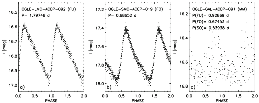
Fig. 5 a Light curve for an LMC AC pulsating in the fundamental mode from the OGLE-IV data set. The ID and the period (days) are labelled. b Same as the left, but for an SMC AC pulsating in the first overtone. c Same as the left, but for the Galactic AC pulsating simultaneously in the first three radial modes. Primary and secondary periods (days) are labelled
