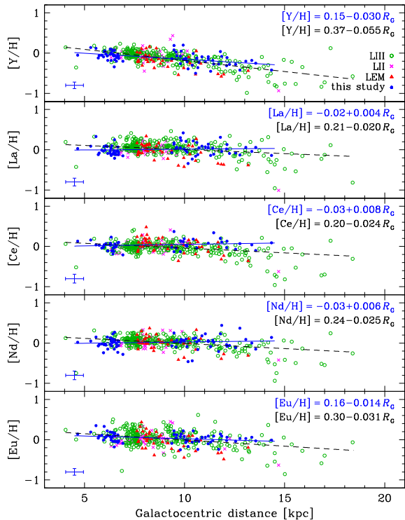
Fig. 27 From top to bottom: Abundances for CCs of neutron capture elements (Y, La, Ce, Nd, Eu) as a function of the Galactocentric distance. Abundances provided by da Silva et al. (2016, filled blue circles) are compared with those of LII (magenta crosses, Luck et al. 2011), LIII (open green circles, Luck and Lambert 2011), and LEM (red triangles, Lemasle et al. 2013). The blue solid line shows the linear regression of our Cepheid sample, while the black dashed line the linear regression of the entire Cepheid sample. The blue error bars display the mean spectroscopic error of the current sample. The abundances available in the literature have similar errors. Adapted from da Silva et al. (2016, Fig. 2). Image credit: R. da Silva
