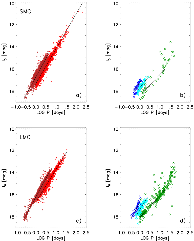
Fig. 16 a Dereddened I -band PL relations for SMC CCs. From shorter to longer periods, the different symbols display FO (dark red) and fundamental (light red) CCs. The solid black lines display the linear fits to the PL relations (see Table S1). b Same as the left, but for FO (dark blue) and FU (light blue) ACs and FU (green) THICs. The black lines display the linear fits to the PL relations (see Table S1). c , d Same as the top, but for LMC Cepheids. Note the increase in sample size of THICs
