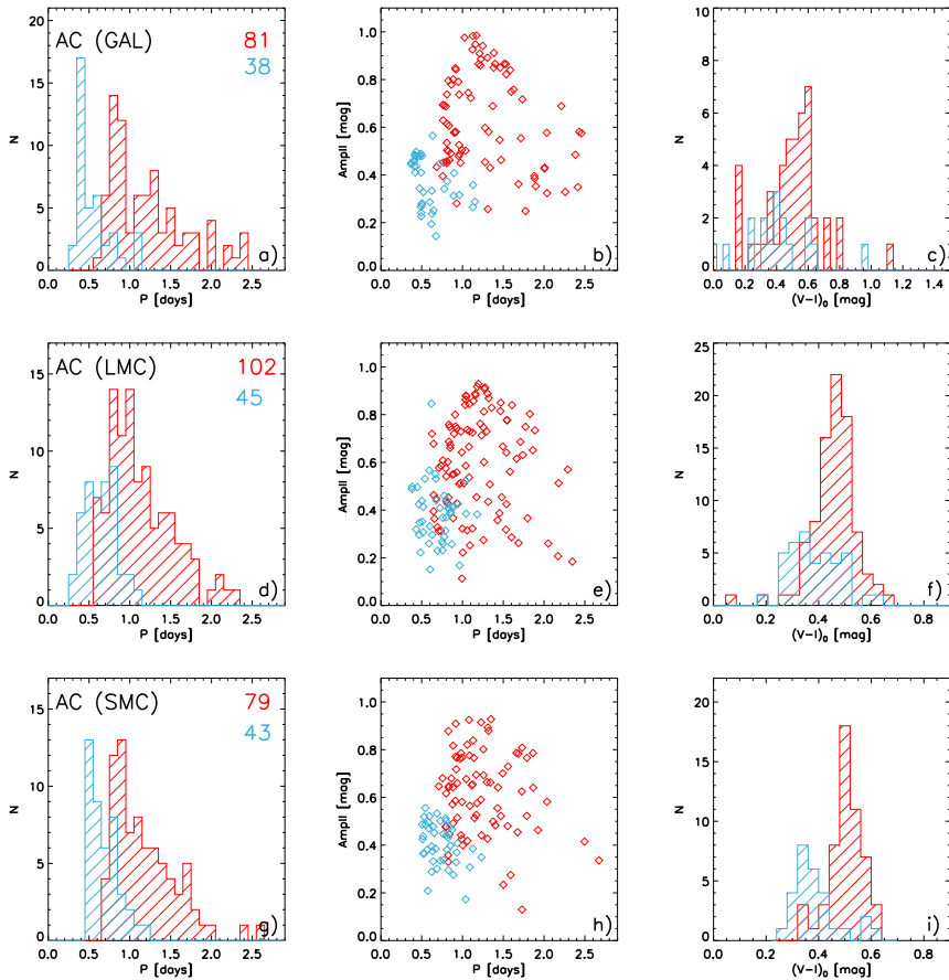
Fig. 6 Top: a Period distribution for fundamental (red-hatched area) and first overtone (light-blue hatched area) Galactic ACs. b I-band luminosity amplitude versus period (Bailey diagram) for both FU and FO ACs. c Dereddened (V - I)_0 color distribution for the same ACs plotted in the left and in the middle panel. Middle: Same as the top, but for LMC ACs. Bottom: Same as the top, but for SMC ACs
