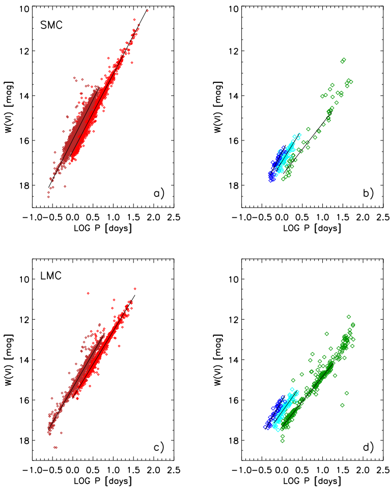
Fig. 17 Top: Optical I , V - I PW relations (see Table S2) for SMC CCs (a) and for ACs plus TIICs (b). Symbols and color coding are the same as in Fig. 16. Bottom: Same as the top, but for LMC Cepheids (CCs (c); ACs plus TIICs (d))
