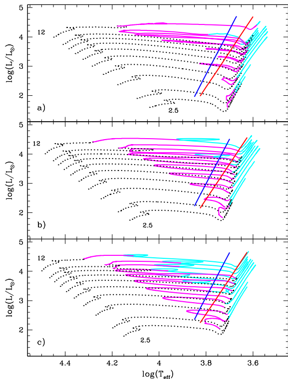
Fig. 4 a Scaled solar evolutionary tracks for young stellar structures computed by neglecting convective overshooting during core hydrogen-burning phases in the Hertzsprung–Russell diagram at fixed chemical composition (metal mass fraction, Z = 0.02 ) and stellar masses ranging from 2.5 to 12 M_{\odot} (see labels). The dashed lines display hydrogen-burning phases, while the magenta color marks central helium-burning phases, the cyan color marks double-shell (H and He) burning phases (Asymptotic Giant Branch). The almost vertical solid lines display the blue (hot, first overtone) and the red (cool, fundamental) edge of the CC instability strip (Fiorentino et al. 2002; De Somma et al. 2021). b Same as a , but for a more metal-poor chemical composition Z = 0.01 . c Same as b , but for a more metal-poor chemical composition Z = 0.001
