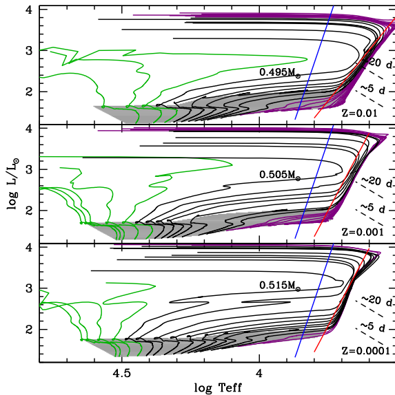
Fig. 10 Top: HRD of HB evolutionary models covering a broad range of stellar masses ( M/M_{\odot} = 0.48\text{--}0.90 ) and the same initial chemical composition ( Z = 0.01 , Y = 0.259 ). The grey area outlines the region between ZAHB (faint envelope) and central-helium exhaustion (bright envelope). The green lines display HB models evolving as AGB-manqué, black lines the post early AGB models, and purple lines the thermal pulsing AGB models (see text for details). The almost vertical blue and red solid lines indicate the hot and cool edge of the TIIC instability strip. The minimum stellar mass (in solar units) crossing the instability strip is labelled in black. The black dashed lines show two iso-periodic lines for 5 and 20 days. Middle: Same as the top panel, but for stellar masses ranging from M/M_{\odot} = 0.4912 to 0.80 and for a metal-intermediate chemical composition ( Z = 0.001 , Y = 0.246 ). Bottom: Same as the top panel, but for stellar masses ranging from M/M_{\odot} = 0.5035 to 0.70 and for a metal-poor chemical composition ( Z = 0.0001 , Y = 0.245 ). Image reproduced with permission from Bono et al. (2020b, Fig. 5), copyright by ESO
