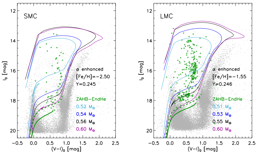
Fig. 15 Left: Comparison between theory and observations in the dereddened I_0 , (V-I)_0 CMD for SMC TIICs. TIICs are marked with light (fundamental) green symbols, while static stars with grey dots. Solid lines display selected HB evolutionary models from the BASTI-IAC database with a \alpha -enhanced chemical composition ( [\text{Fe}/\text{H}] = -2.50 , Y = 0.245 ) and stellar masses ranging from 0.51 M/M_{\odot} to 0.60 M/M_{\odot} (see labelled values). The thick green lines show the Zero Age Horizontal Branch (ZAHB) and the dashed line the end of core helium burning. Right: Same as the left, but for LMC TIICs and more metal-rich HB evolutionary models ( [\text{Fe}/\text{H}] = -1.55 , Y = 0.246 )
