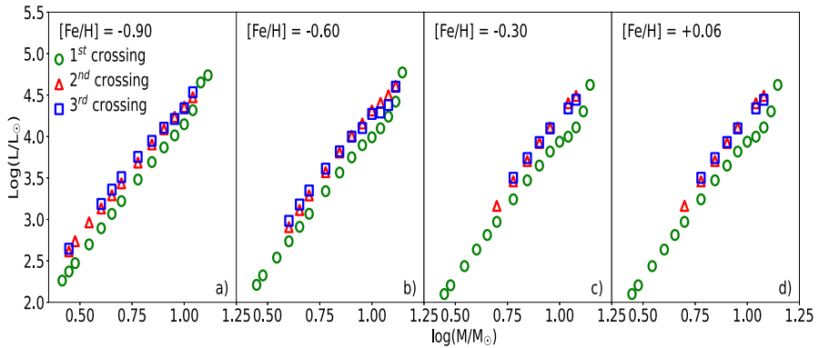
Fig. 22 a Logarithmic stellar mass versus logarithmic luminosity for the different crossings of the instability strip. Predictions plotted in this panel have been computed for a scaled solar mixture and at fixed chemical composition ( [\text{Fe}/\text{H}] = -0.90 ) representative of CCs in metal-poor disk galaxies. The three different crossings are plotted with different colors and symbols. In the less massive regime only the 1st crossing is present, because in these stellar structures the blue loop does not cross the instability strip. In the more massive regime, only the 1st crossing is present because these stellar structures already ignited core helium burning and they cross once the instability strip. b Same as a , but for a chemical composition representative of LMC CCs. c Same as a , but for a chemical composition representative of SMC CCs. d Same as a , but for a chemical composition representative of MW CCs
