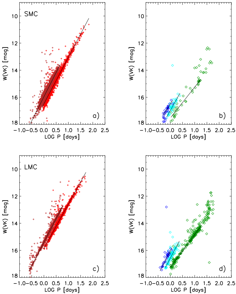
Fig. 18 Top: Optical–NIR K , V - K PW relations (see Table S2 of the Supplementary Information) for SMC CCs (a) and for ACs plus THCs (b). Symbols and color coding are the same as in Fig. 16. Bottom: Same as the top, but for LMC Cepheids (CCs (c) ACs plus THCs (d))
