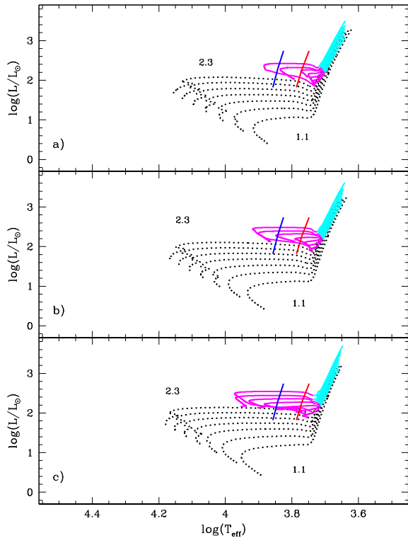
Fig. 7 a Evolutionary tracks for intermediate-age stellar structures in the Hertzsprung–Russell diagram at fixed metallicity ( Z = 0.0008 ) and stellar masses ranging from 1.1 to 2.3 M/M_{\odot} (see labels). The magenta color marks central helium-burning phases, whereas the light blue color marks double-shell (H and He) burning phases (Asymptotic Giant Branch). The almost vertical solid lines display the blue (hot) and the red (cool) edge of the Anomalous Cepheid instability strip (Fiorentino and Monelli 2012; Monelli and Fiorentino 2022). b Same as a , but for Z = 0.0004 . c Same as a , but for Z = 0.0002
