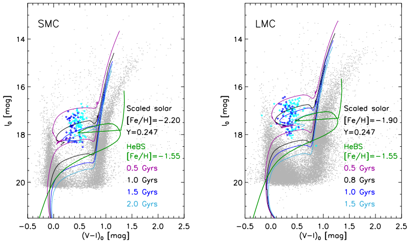
Fig. 14 Left: Comparison between theory and observations in the dereddened I_0 , (V - I)_0 CMD for SMC ACs. ACs are marked with light (fundamental) and dark (first overtone) blue symbols, while static stars with grey dots. Color-coded lines show stellar isochrones from the BASTI-IAC database at fixed chemical composition ( [\text{Fe}/\text{H}] = -2.20 , Y = 0.247 ) and stellar ages ranging from 0.5 Gy to 2 Gy (see labelled values). The green line shows the helium-burning sequence (HeBS) for a more metal-rich ( [\text{Fe}/\text{H}] = -1.55 , Y = 0.248 ) chemical composition. Right: Same as the left, but for LMC ACs and more metal-rich stellar isochrones ( [\text{Fe}/\text{H}] = -1.90 , Y = 0.247 )
