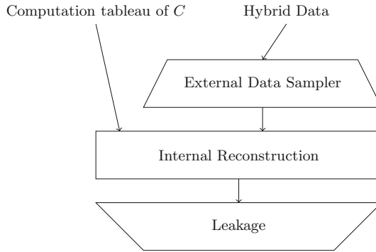
Fig. 4. Components of the security proof. When the external sampler is given, the input data for \text{Hybrid}_0 , the adversary's view is identical to the output of the transformed circuit as in the real world. In \text{Hybrid}_3 , the adversary's view is identical to the output of the simulator as in the ideal world. Indistinguishability of consecutive hybrids is argued by analyzing the view of the leakage function composed with Internal Reconstruction.
