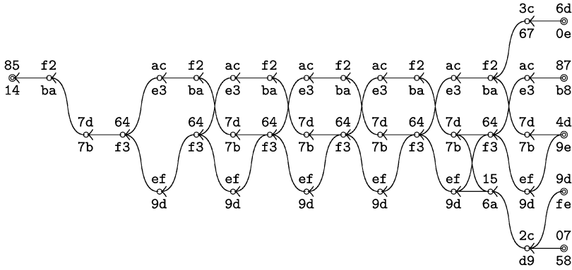
Fig. 1. Graph of solutions of (11) for k = 256 and a/b = 11/19 .
