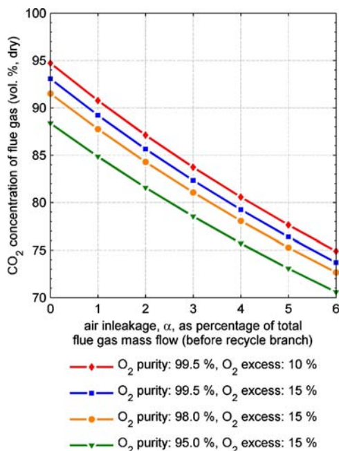
Fig. 8 Influence of the different sources of impurities on the CO 2 concentration that can be achieved in the dry flue gas
