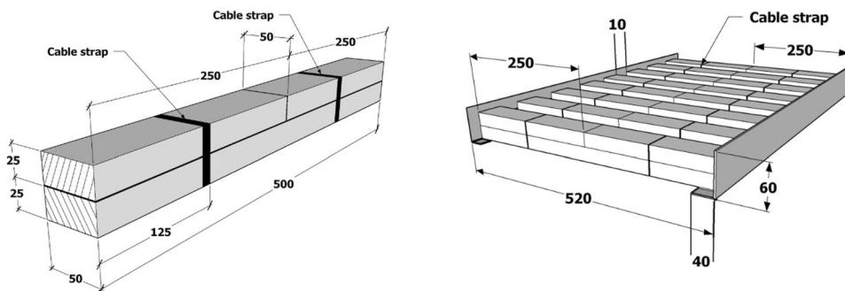
Fig. 1 Configuration of Bundle test specimens. Left: Specimen consisting of three members held together by cable straps. Right: Exposure of bundle test specimens on aluminium L-profiles
