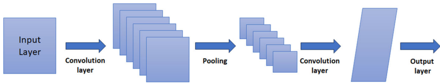
Fig. 6 CNN architecture
