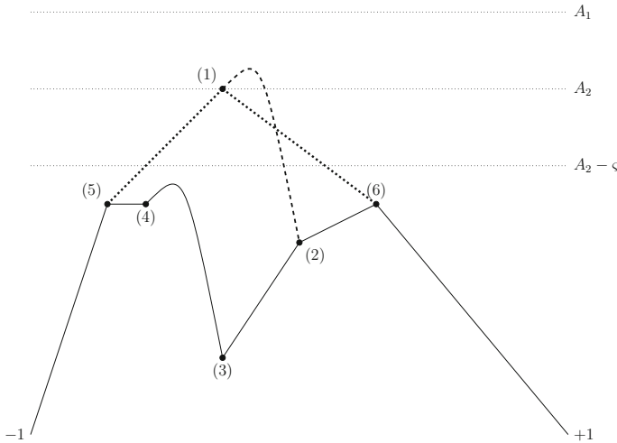
FIGURE 2. The Paths. To prove V_0 = 0 , we follow the path from -1 to (5) , then the dotted line to (1) , dotted line to (6) , then complete the path to +1 . The dashed line from (1) to (2) is the construction of the competitor. Then, to prove that M is embedded, we follow the path from -1 to +1 given by the solid lines. Refer to Fig. 3 for the local picture about the non-embedded point z_0 at each numbered stage on the paths
