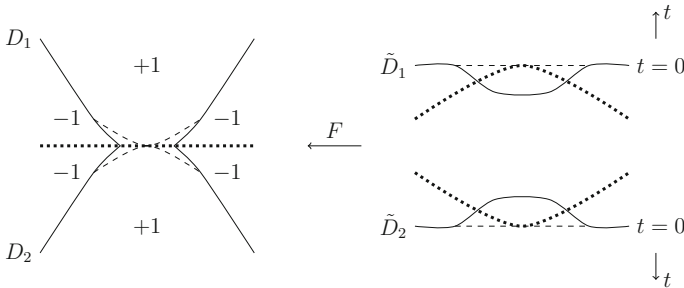
FIGURE 5. How the competitor is constructed as the graph of bump functions about points x_0^1 and x_0^2 over \tilde{M} . Whatever is bumped out beyond the dotted line, on the right-hand side, is not considered in N . In other words, it is deleted
