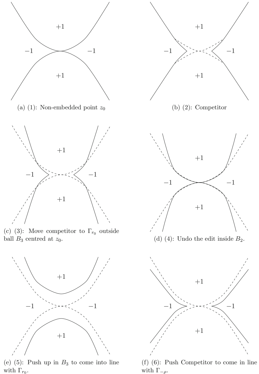
FIGURE 3. Stages of the Path at the non-embedded point z_0 . In each image, the dashed lines represent the original \lambda -CMC disks, as a reference to what we are changing at each step. Furthermore, in each image, it is the solid lines that are the boundaries between the '+1' and '-1' regions
