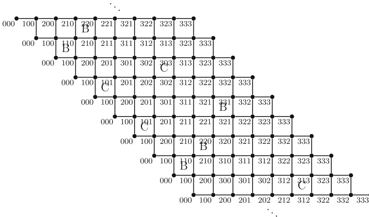
Fig. 9 A decorated growth diagram for a Kreweras word
