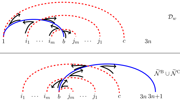
Fig. 6 Figure illustrating the proof of Lemma 3.10
