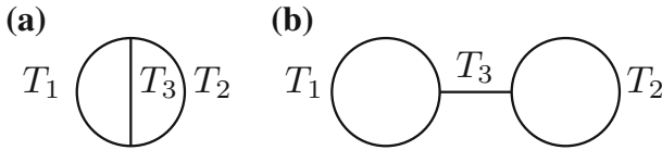
FIGURE 4. Genus-two graphs described in the examples
