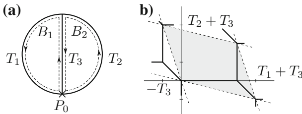
FIGURE 3. a Genus-two graph with edges lengths T_1, T_2, T_3 . b Image of \Gamma (thick line) by the tropical Abel–Jacobi map in the Jacobian J(\Gamma) = \mathbb{R}^2 / \mathbf{K}^{(2)}\mathbb{Z}^2
