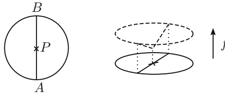
FIGURE 5. Example of rational function f on a two-loop graph
