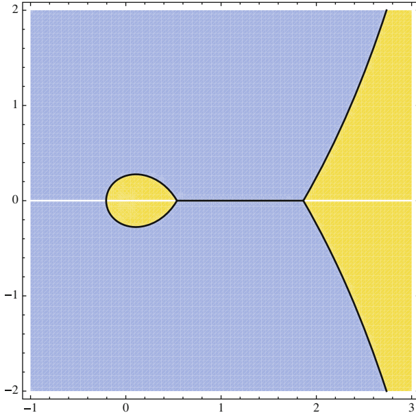
FIGURE 5. The real part of the Penner holomorphic effective potential in the complex z -plane, for t = 0.1 . In blue is the region \Re V_{h;\text{eff}}^{\text{P}}(z) < 0 , in yellow the region \Re V_{h;\text{eff}}^{\text{P}}(z) > 0 , and the black lines correspond to the Stokes lines \Re V_{h;\text{eff}}^{\text{P}}(z) = 0 (which also include the cut of the spectral curve). The white cuts corresponds to the logarithmic branch cuts (color figure online)
