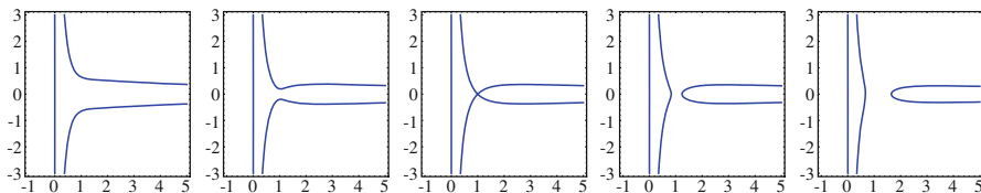
FIGURE 6. The Stieltjes–Wigert algebraic curve for values of t = -0.1, -0.01, 0, +0.01, +0.05 , from left to right , respectively. Notice that the algebraic curve is singular for t = 0
