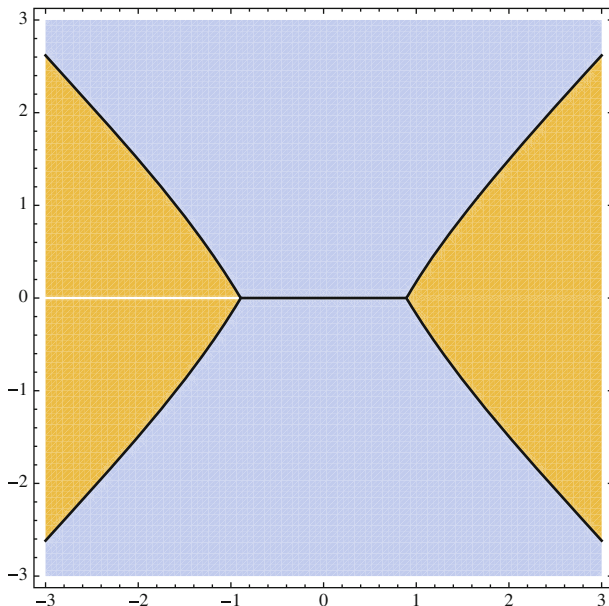
FIGURE 3. The real part of the Gaussian holomorphic effective potential in the complex z -plane, for t = 0.2 . In blue is the region \Re V_{h;\text{eff}}^G(z) < 0 , in orange the region \Re V_{h;\text{eff}}^G(z) > 0 , and the black lines correspond to the Stokes lines \Re V_{h;\text{eff}}^G(z) = 0 (which also include the cut of the spectral curve). The white cut corresponds to the logarithmic branch cut (color figure online)
