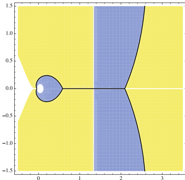
FIGURE 7. The real part of the Stieltjes–Wigert holomorphic effective potential in the complex z -plane, for t = 0.1 . The black lines correspond to the Stokes lines \Re V_{h;\text{eff}}^{\text{CS}}(z) = 0 (which also include the cut of the spectral curve). The white cuts and regions correspond to the logarithmic and dilogarithmic branch cuts. Because of the choice of principal sheets in Mathematica the colored regions are now not so clear. Akin to the Penner model, the region in yellow , to the right of the vertical black lines , and the region in blue , inside the “closed bubble”, have \Re V_{h;\text{eff}}^{\text{CS}}(z) > 0 , in the principal sheet. The rest is \Re V_{h;\text{eff}}^{\text{CS}}(z) < 0 (color figure online)
