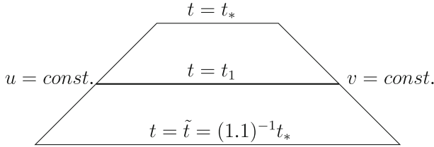
FIGURE 4. The region \mathcal{P}
