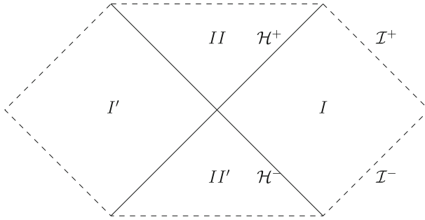
FIGURE 1. Schwarzschild spacetime
