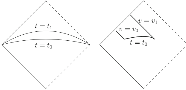
FIGURE 2. Regions of integration
