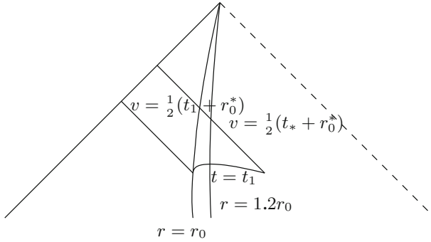
FIGURE 3. The region \mathcal{R}
