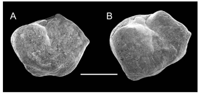
Fig. 6. Palaetoinca sp. otoliths (left lapilli), Upper Marine Molasse (Karpatian), Mauensee, central Switzerland. A, B) Dorsal view, mirrored (BSPG 2003 XVIII 90–91). SEM pictures. Scale bar: 0.5 mm.
