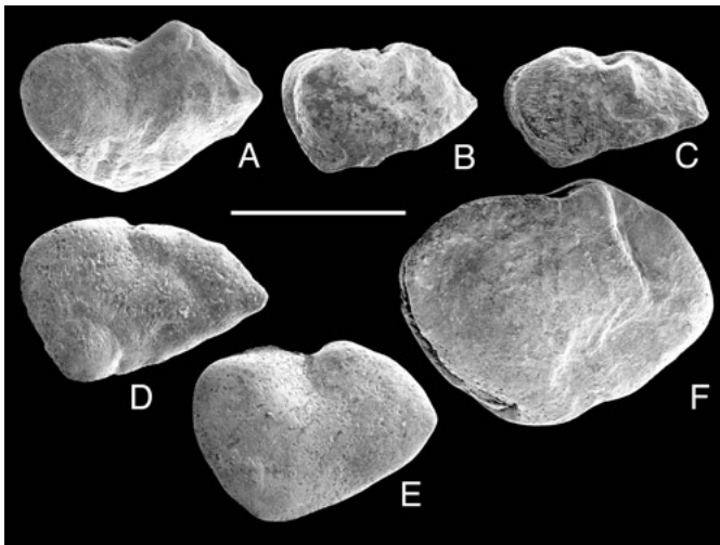
Fig. 4. Palaocarassius sp. otoliths (lapilli), Upper Marine Molasse (Karpatian), Mauensee, central Switzerland. A) Right lapillus in dorsal view (BSPG 2003 XVIII 78). B, C) Right lapilli in ventral view, mirrored (BSPG 2003 XVIII 79–80). D, E) Left lapilli in dorsal view, mirrored (BSPG 2003 XVIII 81–82). F) Left lapillus in ventral view (BSPG 2003 XVIII 83). SEM pictures. Scale bar: 1 mm.
