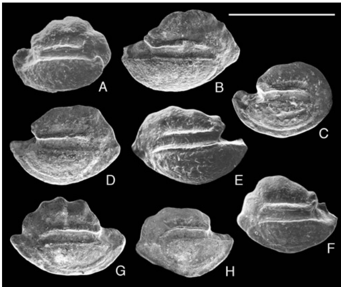
Fig. 9. Hemitrichas martinii (REICHENBACHER 1993) otoliths (sagittae), Upper Marine Molasse (Karpatian), Mauensee, central Switzerland. A–D) right sagittae (BSPG XVIII 100–103). E–H) left sagittae (BSPG XVIII 104–107). SEM pictures. Scale bar: 1 mm.
