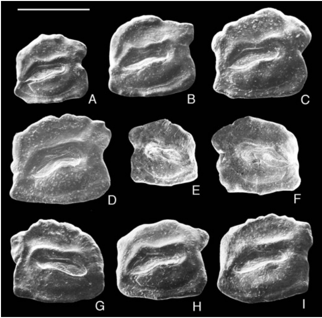
Fig. 15. Gobius aff. multipinnatus (MEYER 1852) otoliths (sagittae), Upper Marine Molasse (Karpatian), Mauensee, central Switzerland. A–D, H, I) Right sagittae (BSPG XVIII 159–162, 166–167). E–G) Left sagittae (BSPG XVIII 163–165). SEM pictures. Scale bar: 1 mm.
