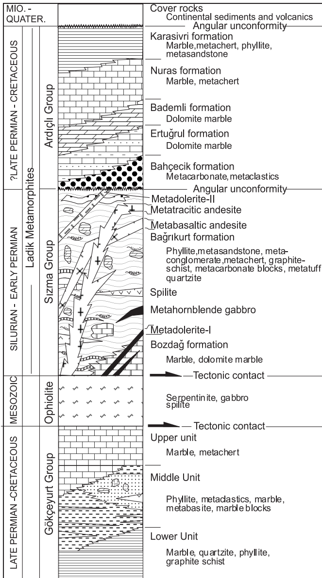
Fig. 3. Generalized tectono-stratigraphic section of the studied area.
