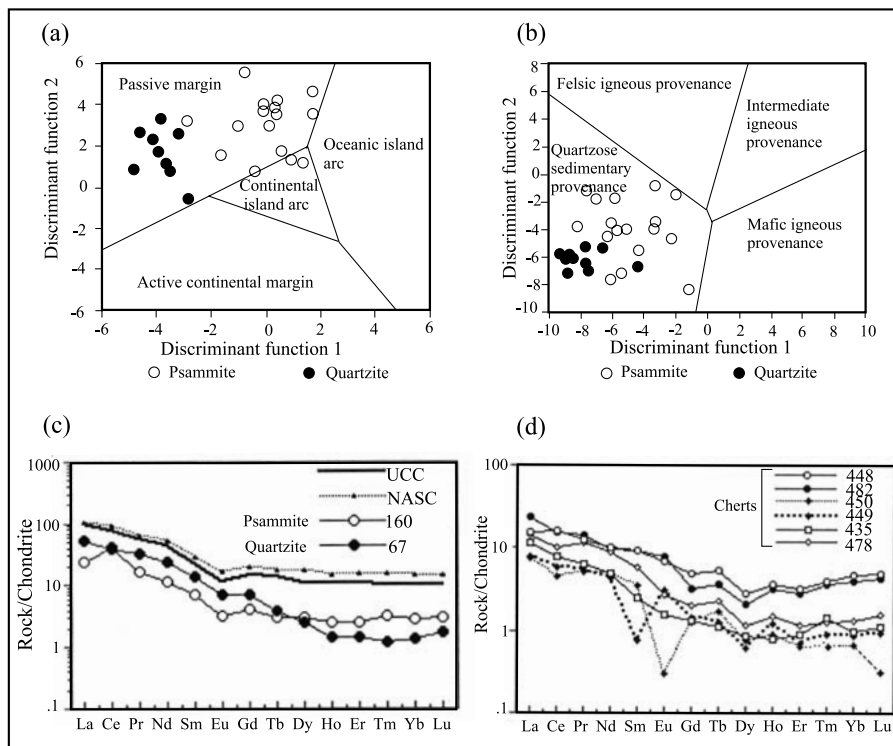
Fig. 4. (a) Plot of discriminant functions F1 and F2 (Bhatia, 1983) showing the position of psammite and quartzite from Devonian – Early Permian Bağrıkturt formation. (b) Plot of discriminant function F1 and F2 (Roser & Korsch 1988) showing the provenance of psammite and quartzite. (c) Chondrite normalised REE patterns for psammite (160) and quartzite (67) (UUC; upper continental crust, NASC; North American shale composition) (after Boynton 1984). (d) Chondrite-normalised rare earth element distribution patterns for metacherts from the Kadınhanı area. Chondrite normalising values from Boynton (1984).
