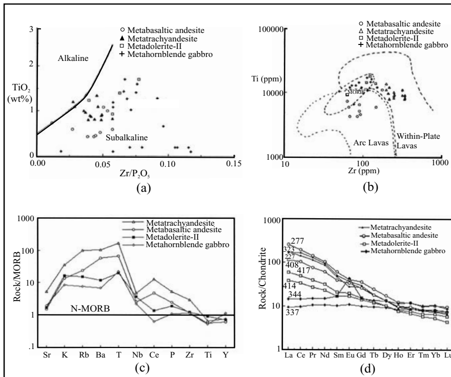
Fig. 7. (a) Zr/P2O5 versus TiO2 plot used to reveal the magma type. Field boundaries from Floyd & Winchester (1975) and Winchester & Floyd (1976). (b) Ti vs. Zr plot for the meta-igneous rocks of the Kadınhanı area. Field boundaries from Pearce (1982) and Pharaoh & Pearce (1984). (c) MORB-normalized incompatible element patterns for averages of the meta-igneous rocks. Normalizing values are as cited in Pearce (1982). (d) Chondrite-normalized rare earth element patterns for meta-igneous rocks. Chondrite normalizing values are from Boynton (1984). All analytical data are derived from Kurt 1996 and 1997.
