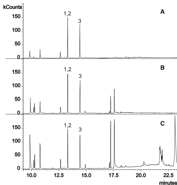
Fig. 1 GC-MS chromatograms of standards solution at the concentration of 40 ng mL -1 (a), fortified sample (50 µg kg -1 ) cleaned-up with 300 mg PSA (b), fortified sample (50 µg kg -1 ) cleaned-up with 300 mg celite (c); 1, 3-MCPD-d 5 , 2, 3-MCPD, 3, 3-MBPD
