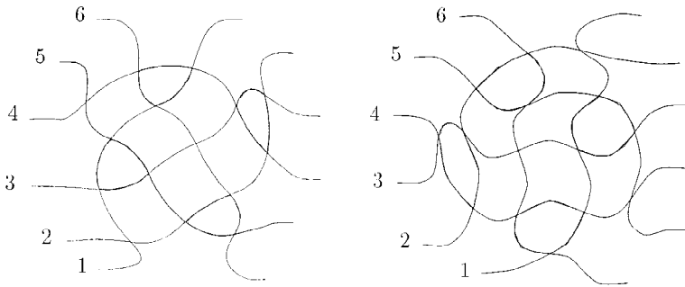
Fig. 3. Two arrangements \mathcal{A}_1 and \mathcal{A}_2 with corresponding triangular faces.
