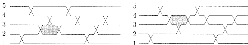
Fig. 1. Elementary flip at the shaded triangle.
