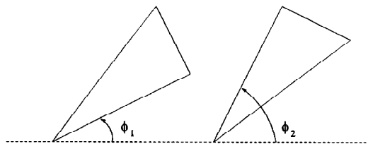
Fig. 8. Orientation of triangles.
