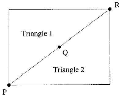
Fig. 7. A fault line.
