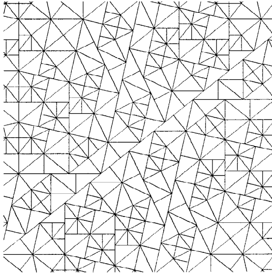
Fig. 1. Part of the tiling Til(1/2) .
