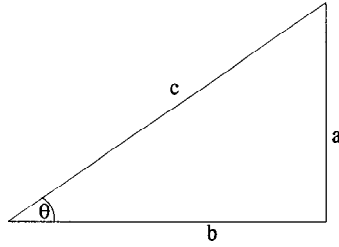
Fig. 2. The basic triangle.
