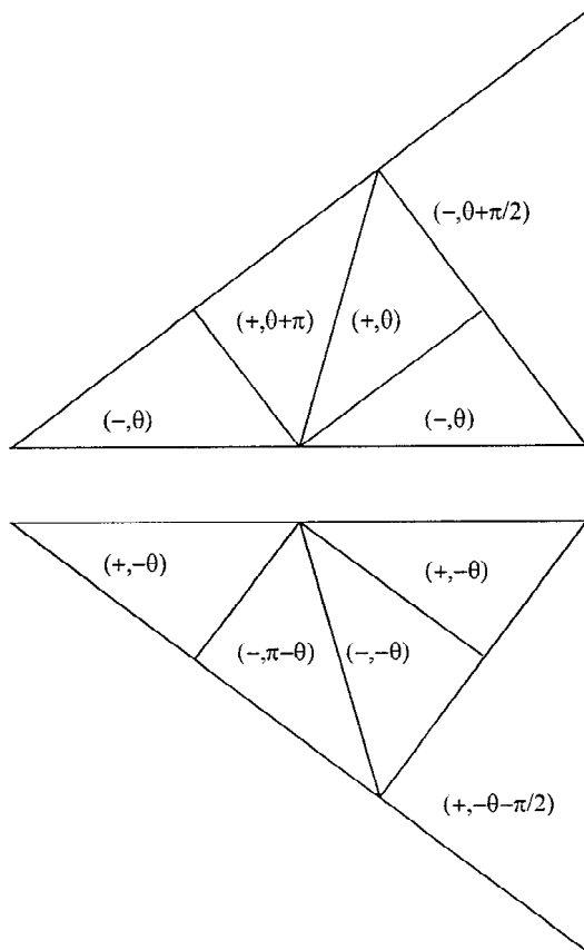
Fig. 9. Orientation of daughter tiles.
