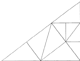
Fig. 4. Two subdivisions of a triangle with a > b/2 .
