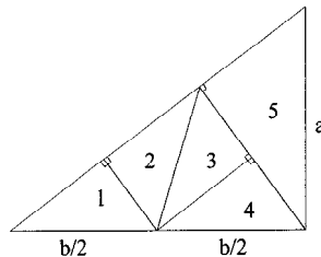
Fig. 3. The substitution rule.
