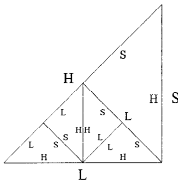
Fig. 11. “Long” and “short” edges in Til(1/3) .
