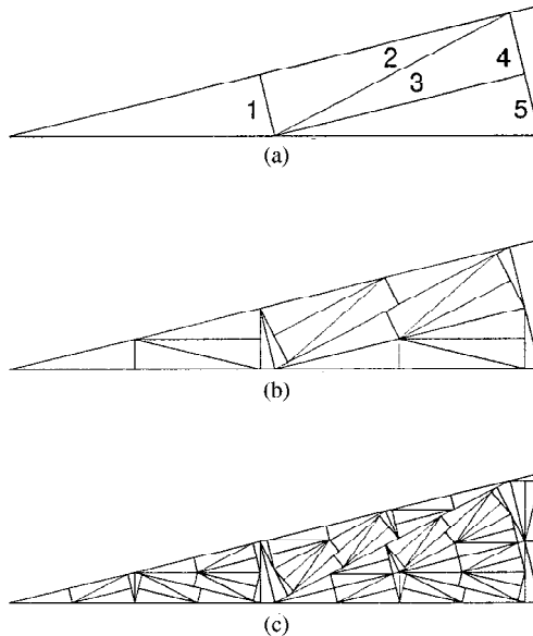
Fig. 10. Three stages of subdivision for Til(2) .
