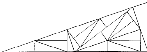
Fig. 5. Two subdivisions of a triangle with a < b/2 .
