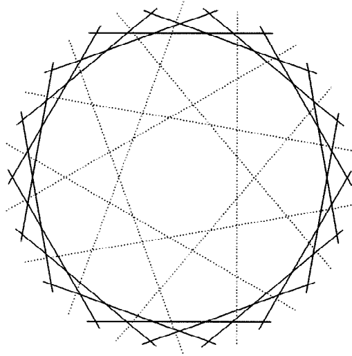
Fig. 2. The family of segments \mathcal{S}_1 .
