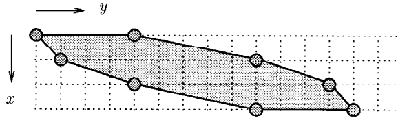
Fig. 1. The subset P of the 2^2 \times 2^4 grid.
