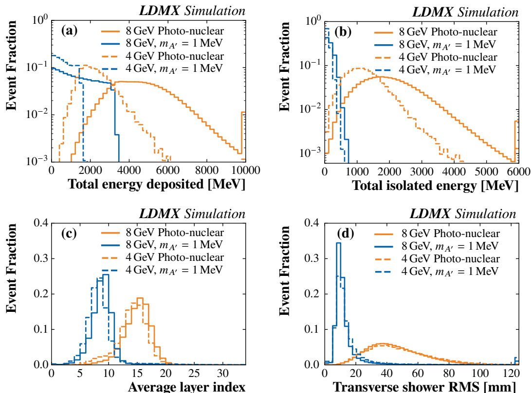
Figure 5. Distributions of key variables for dark photon signal events (blue) and ECal PN background events (orange) at 8 GeV (solid) and 4 GeV (dashed). All distributions are normalised to the number of events in the respective sample after the trigger requirement. (a) The summed energy of all ECal hits. Due to the experimental resolution, the total energy can sometimes exceed the energy of the incoming beam electron. (b) The energy in isolated hits, with no energy deposits in neighboring ECal cells. (c) The energy-weighted average hit layer number. (d) The transverse spread of energy depositions in the ECal. The rightmost bins are overflow bins.
