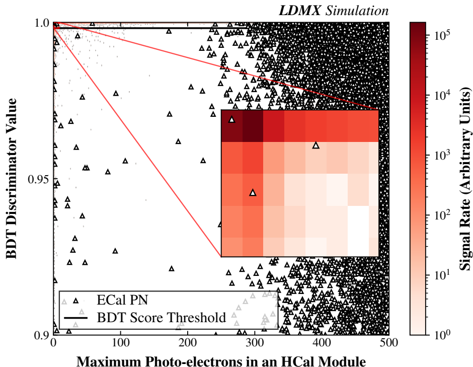
Figure 20. Distribution of BDT discriminator values and maximum photo-electrons in the HCal, in ECal photo-nuclear events. The inset shows the signal region. The rate of m_{A'} = 1000 MeV signal events is shown underneath.
