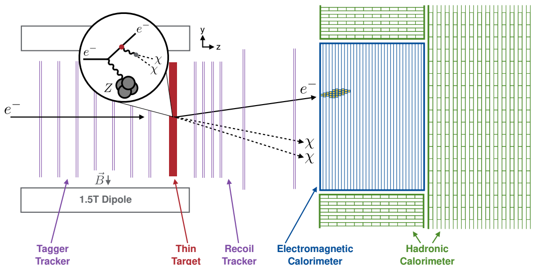
Figure 2. A diagram of the LDMX detector apparatus, illustrating production of DM in the target from a scattering beam electron, and the corresponding response of the various sub-systems to the missing-momentum signature. The drawing is not to scale.
