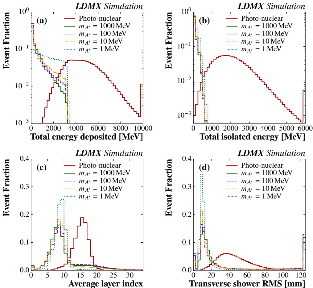
Figure 18. Distributions of selected BDT variables at 8 GeV, comparing signal events of various mediator masses and ECal photo-nuclear events. (a) The sum of the energy in each ECal cell. The effect of the trigger is seen in the steep drop in signal events around 3160 MeV, while photo-nuclear events often deposit energy deeper in the ECal. (b) Sum of energy in ECal cells for which neighbouring cells in the same layer have no activity. (c) Average layer index of ECal hits. (d) Energy-weighted RMS of ECal hit’s transverse distance from the energy centroid. The rightmost bins are overflow bins.
