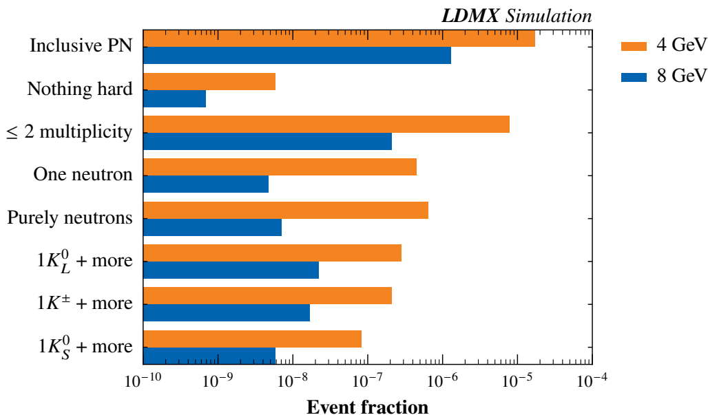
Figure 4. Classification of daughter particles from bremsstrahlung photon PN interactions in the ECal based only on particles with at least 200 MeV kinetic energy. Events passing the trigger are shown as a fraction of EoT. The kaon rows consider exactly one kaon and any number of other particles, and the categories are not required to be exclusive.
