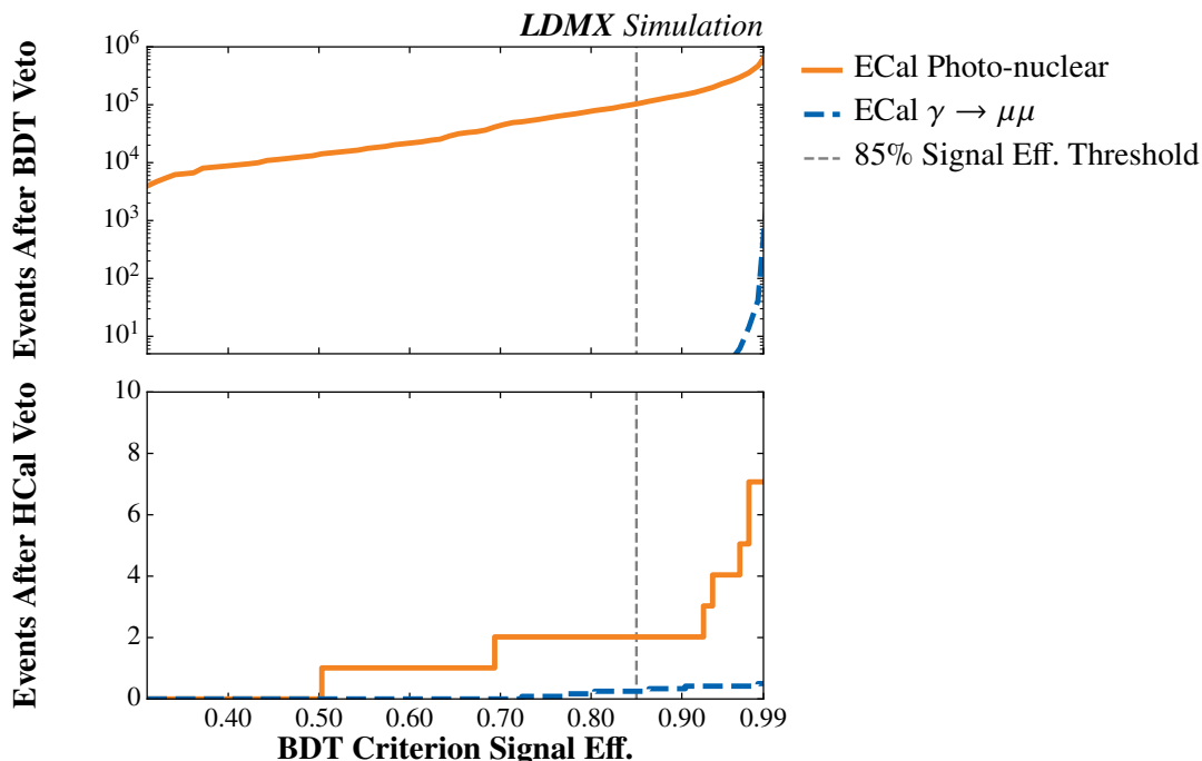
Figure 14. The number of events passing up to and including the BDT discriminator value threshold (above) and additionally the HCal activity requirement (below), depending on the chosen BDT signal efficiency for m_{A'} = 1 MeV. Both the ECal PN sample (orange) and the ECal \gamma \rightarrow \mu\mu sample (blue) reach zero events remaining with sufficiently loose signal efficiency requirements. Both backgrounds are scaled to 2 \times 10^{14} EoT in this figure. The performance with an 85% signal efficiency requirement is marked by the intersections with the dashed grey line.
