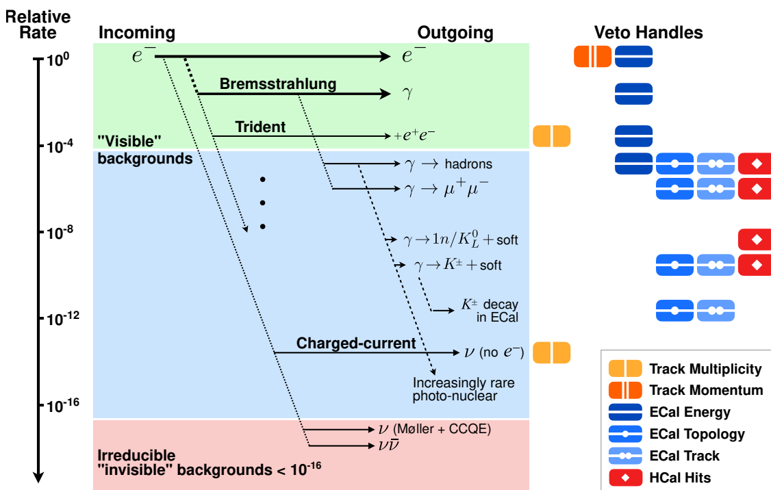
Figure 3. Relative rates of background processes at 8 GeV beam energy, along with the veto handles used to reject them, down to a relative rate of < 10^{-16} . The colour shading groups different background classes: the upper green section corresponds to events in which the full beam energy is deposited in the ECal; the middle blue section is rarer reactions resulting in anomalous energy depositions in the ECal or particles escaping the ECal; and the bottom red section corresponds to irreducible backgrounds with real missing energy.
