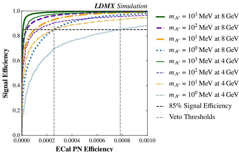
Figure 11. Relationship between background efficiency (of the ECal PN background) and the signal efficiency for different dark photon mediator masses m_{A'} . Thicker lines show the performance at 8 GeV, thinner lines at 4 GeV. The two vertical dashed grey lines show the background rejection power at 8 GeV and 4 GeV, from left to right respectively, that maintains at least 85% signal efficiency across the m_{A'} mass range.
