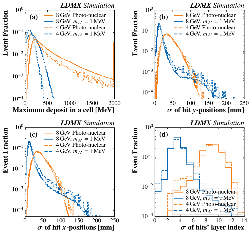
Figure 17. Distributions of selected BDT variables, comparing signal events with m_{A'} = 1 MeV and ECal photo-nuclear events, at both 4 GeV and 8 GeV beam energy. (a) The largest energy deposit made to any one ECal cell. (b) Standard deviation of all ECal hit's y -position. (c) Standard deviation of all ECal hit's x -position. (d) Standard deviation of all ECal hit's layer index. The rightmost bins are overflow bins.
