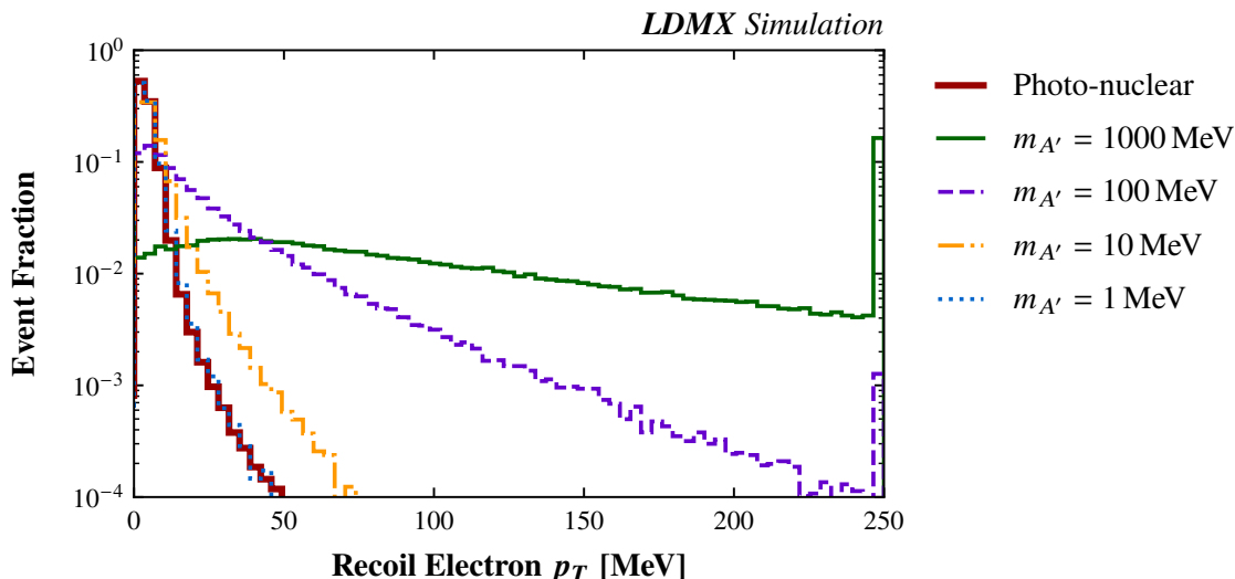
Figure 6. p_T distribution of the recoiling electron in an 8 GeV beam, in events passing the missing energy trigger, for dark photon signal events at various mediator masses m_{A'} , and background events with photo-nuclear reactions in the ECal. The rightmost bin is an overflow bin.
