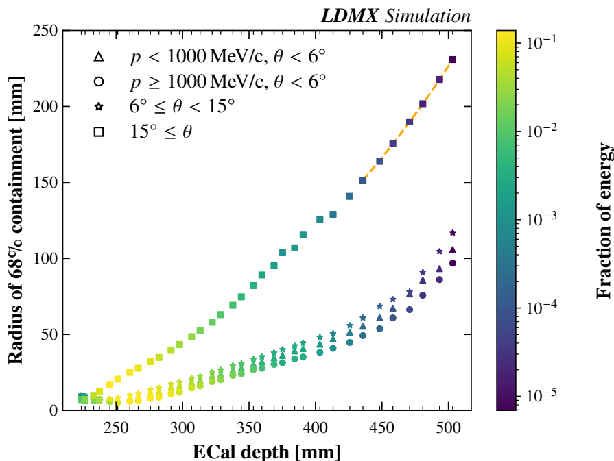
Figure 8. The containment radius in each ECal layer is defined as the radius containing on average 68% of a signal electron’s electromagnetic shower. The phase space of electron momentum p and electron angle to the beamline at the target \theta is split into four regions, corresponding to the four curves. In the last five layers for the high angle electrons, a polynomial fit is used to extrapolate the containment radii due to low statistics. The relative distribution of energy between layers, in a certain category of radii, is expressed by the color of the scattered points.
