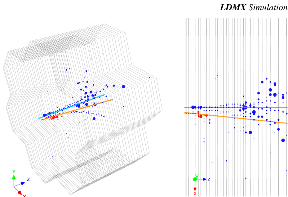
Figure 7. Event display of ECal activity for a photo-nuclear event vetoed by the BDT. A small electron shower (red) is deposited in the first few ECal layers along the expected trajectory of the recoil electron (orange). Proton and charged pion showers (blue) induced by the bremsstrahlung photon are deposited deeper in the ECal, with significant deposits seen near the expected photon trajectory (cyan).
