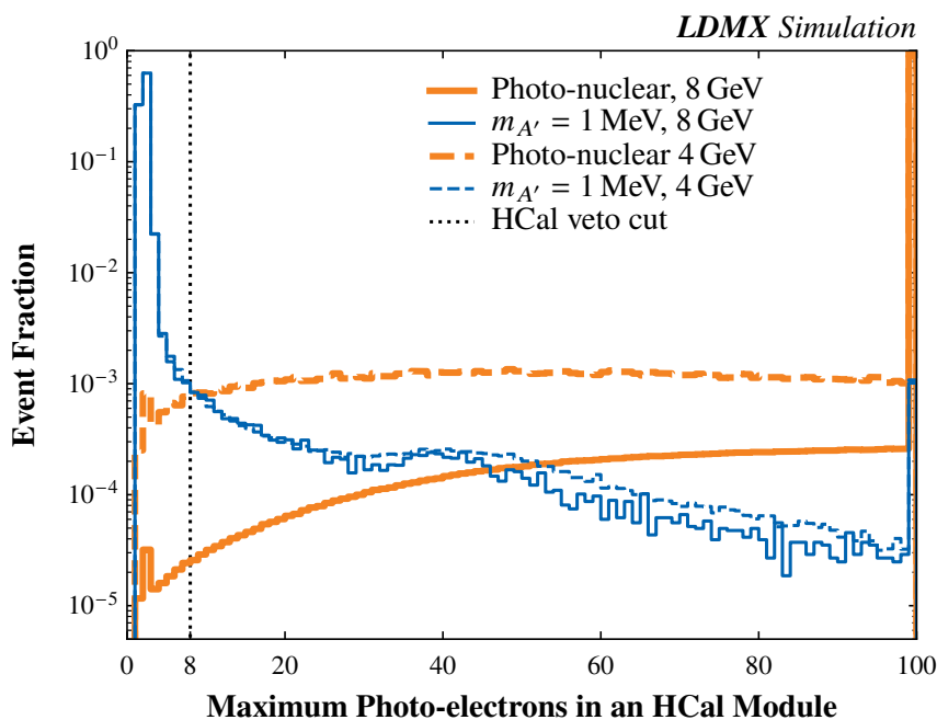
Figure 12. The maximum number of photo-electrons measured in any HCal bar, in events passing only the missing energy trigger veto, at both beam energies of 4 GeV (dashed lines) and 8 GeV (solid lines). Photo-nuclear backgrounds are shown in orange, and the signal for a 1 MeV dark photon in blue. The rightmost bin is an overflow bin.
