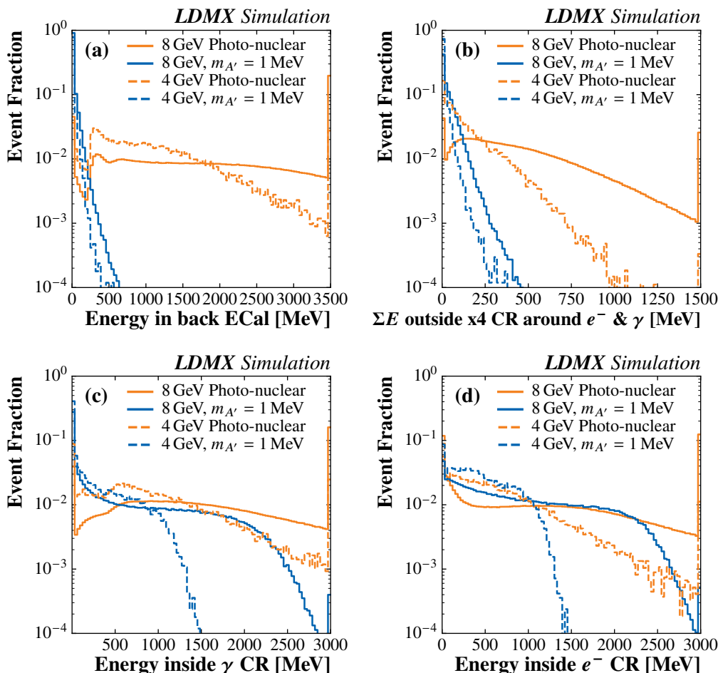
Figure 16. Distributions of selected BDT variables, comparing signal events with m_{A'} = 1 MeV and ECal photo-nuclear events, at both 4 GeV and 8 GeV beam energy. (a) Total energy in the last 14 ECal layers. (b) Total energy in cells more than four containment radii away from the projected recoil electron and bremsstrahlung photon trajectories. (c) Total energy in cells within one containment radii around the projected bremsstrahlung photon trajectory. (d) Total energy in cells within one containment radii around the projected recoil electron trajectory. The rightmost bins are overflow bins.
