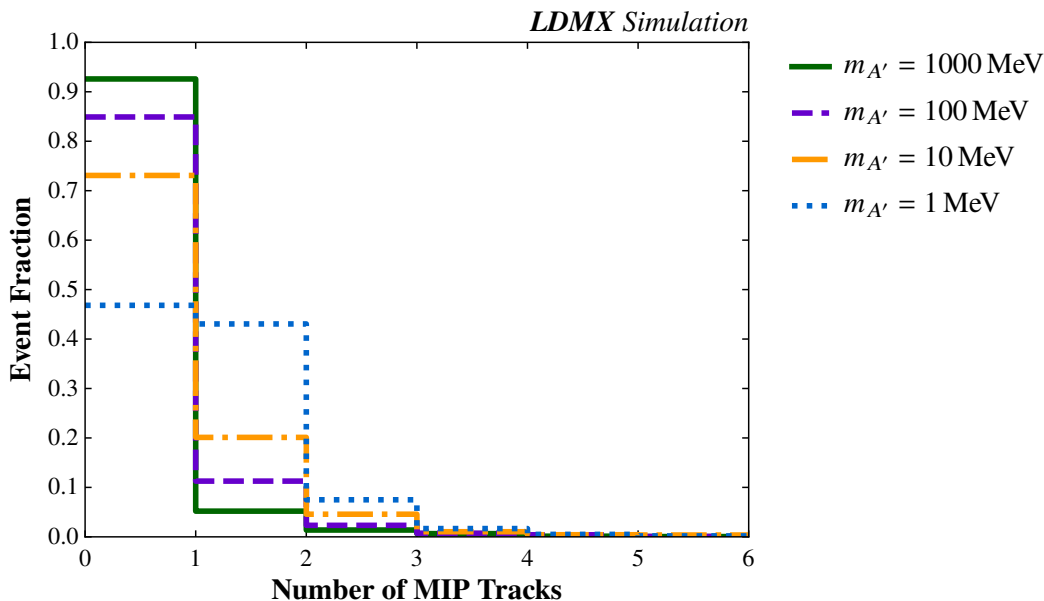
Figure 15. The number of MIP tracks found in signal events that pass all previously described vetoes, at various mediator masses.
