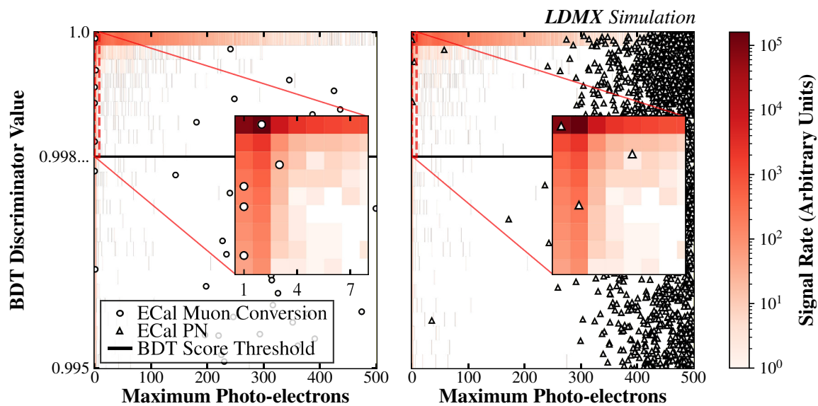
Figure 13. Distribution of BDT discriminator values and maximum number of photo-electrons in the HCal, in muon conversion (left) and photo-nuclear (right) events in the ECal, near the signal region. The insets show the signal region, where a few events in both background classes pass both the BDT and HCal vetos. The signal rate for m_{A'} = 1000 \text{ MeV} is shown underneath.
