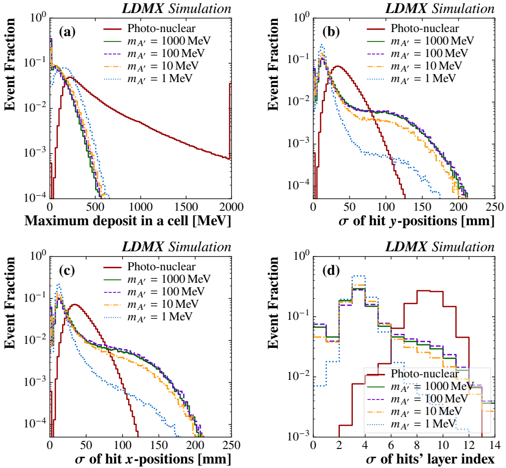
Figure 19. Distributions of selected BDT variables at 8 GeV, comparing signal events of various mediator masses and ECal photo-nuclear events. (a) The largest deposit made to any one ECal cell. (b) Standard deviation of ECal hit's y -position. (c) Standard deviation of ECal hit's x -position. (d) Standard deviation of ECal hit's layer index. The rightmost bins are overflow bins.
