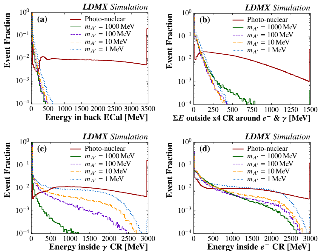
Figure 9. A selection of BDT input variables. (a) Energy in the last 14 ECal layers. (b) The total energy (in all ECal layers) outside four times the containment radii around the electron and bremsstrahlung photon trajectories. (c) The energy within the containment radii around the photon bremsstrahlung photon trajectory, summed over all ECal layers. (d) The energy within the containment radii around the electron trajectory, summed over all ECal layers. The rightmost bins are overflow bins.
