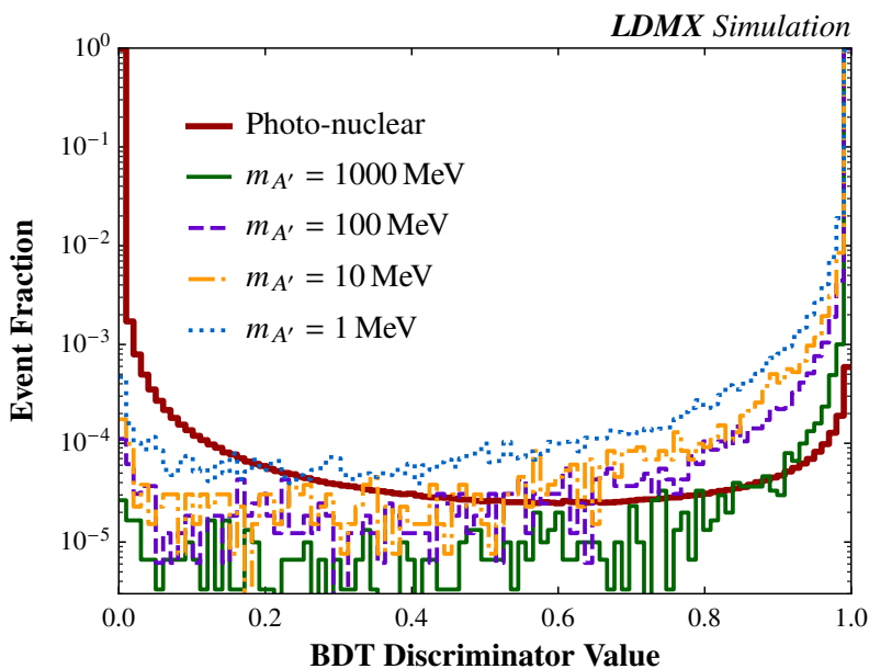
Figure 10. BDT scores assigned to ECal photo-nuclear background events and signal events for various mediator masses.
