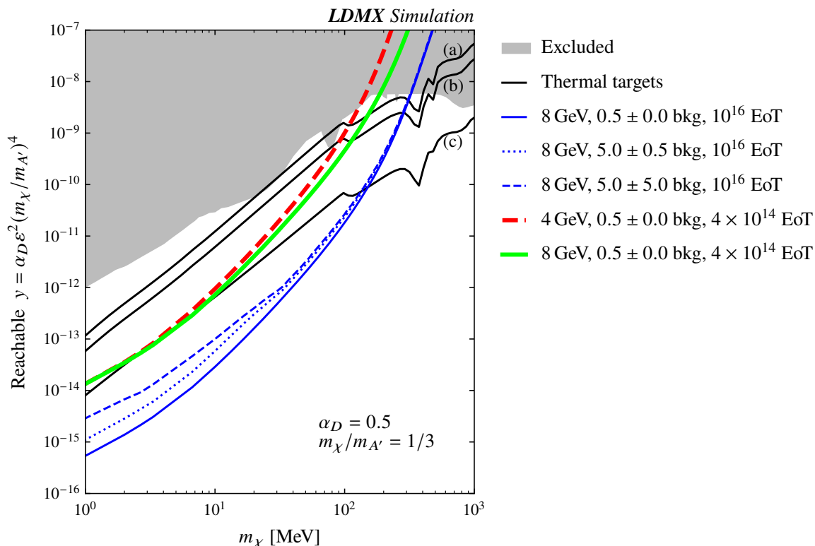
Figure 1. The projected reach of LDMX in the dark bremsstrahlung model at 4 and 8 GeV beam energies. Several scenarios are shown for the 10^{16} electrons on target (EoT) run at 8 GeV assuming different background levels. Three thermal relic targets are shown as black lines, corresponding from top to bottom, (a) to scalar, (b) Majorana fermion, and (c) Pseudo-Dirac fermion models of DM [2]. The region in grey is already excluded by other experiments [9–16]. A 50% signal efficiency is assumed across the entire m_\chi mass spectrum at both beam energies.
