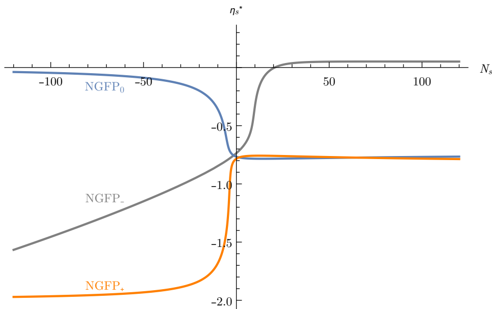
Figure 6. Fixed point value of the scalar anomalous dimension \eta_s^* evaluated for the three classes of fixed points \text{NGFP}_- , \text{NGFP}_0 , and \text{NGFP}_+ as a function of N_s .
