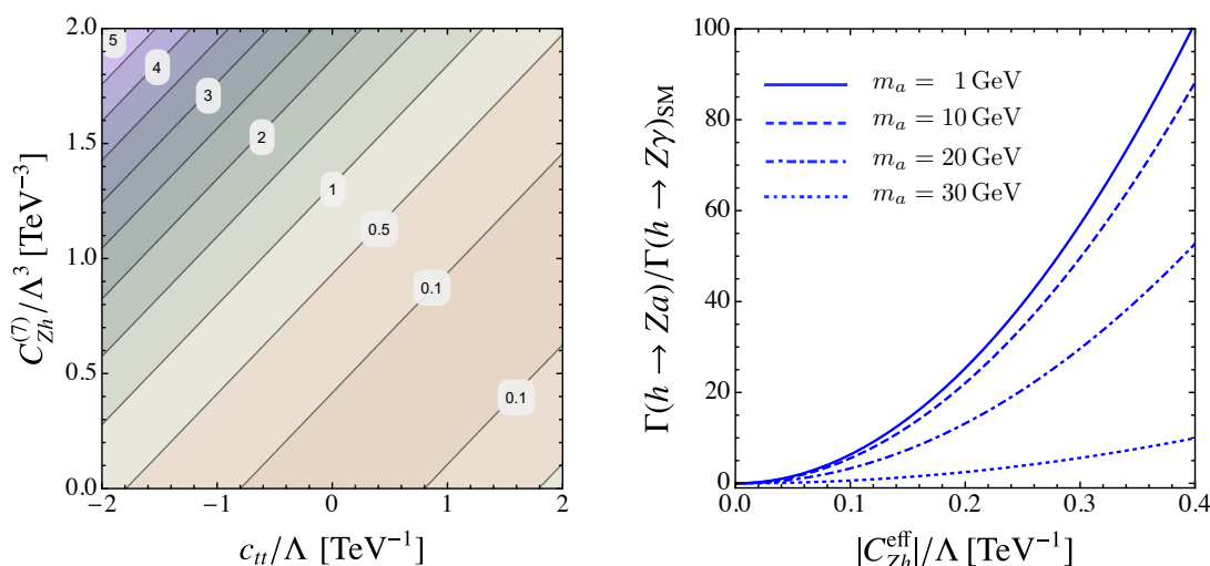
Figure 11. Left: contours for the ratio \Gamma(h \rightarrow Za)/\Gamma(h \rightarrow Z\gamma)_{SM} in the plane of the Wilson coefficients c_{tt} and C_{Zh}^{(7)} for m_a < 1 GeV and \Lambda = 1 TeV. Right: the same rate ratio as a function of the effective Wilson coefficient C_{Zh}^{eff} for different ALP masses.
