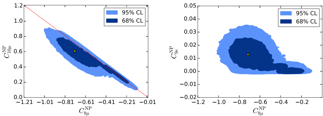
Figure 3. Allowed regions at 68% and 95% CL from the global fit for the Wilson coefficients of b \rightarrow sl^+ \ell^- transitions. The best fit point is illustrated with a star. The red line on the left plot illustrates the correlation C_{9\mu}^{\text{NP}} = -C_{10\mu}^{\text{NP}} .
