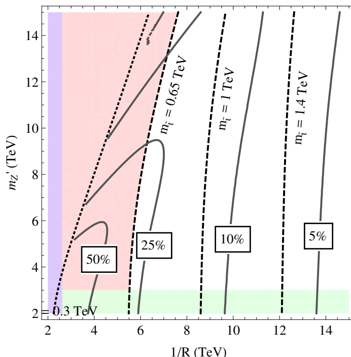
Figure 9. Fine-tuning \Delta^{-1} (solid lines) as a function of 1/R and the Z' mass, eq. (4.12). Iso-contours of stop mass are dashed. Limits from LHC8 searches for \tilde{t} \rightarrow t + \text{MET} [98, 99] (red) and Z' resonance searches [96, 97] (green) are shaded. Subdominant limits m_{\tilde{g}} \approx 1/(2R) \gtrsim 1.3 TeV from \tilde{g} \rightarrow t\bar{t}/b\bar{b} + \text{MET} searches (blue) are also shaded [100, 101].
